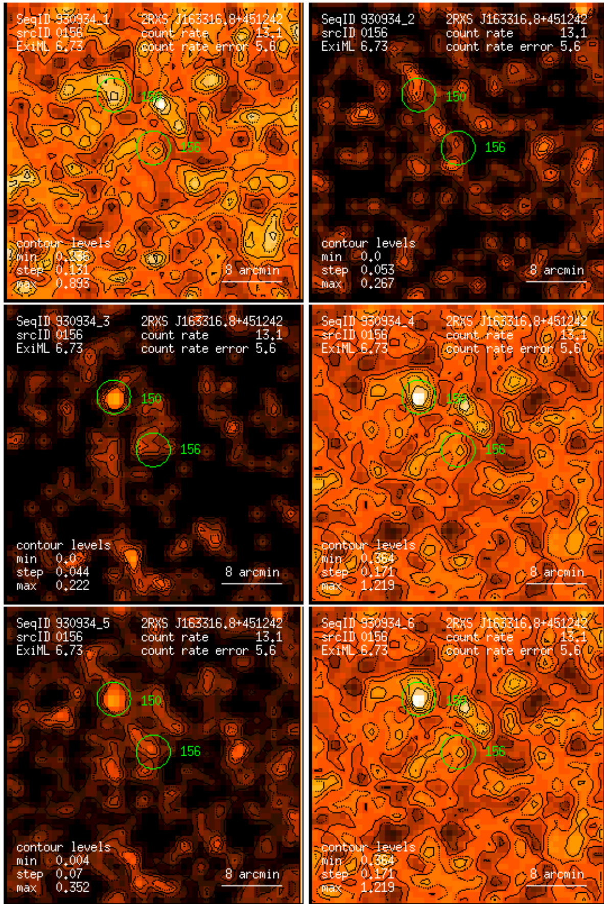
Figure 156: RASS 930934: detection 0156: band rate images, Gaussian filter: (1) PSPC channels 11 – 41, (2) 52 – 90, (3) 91 – 201, (4) 11 – 235, (5) 52 – 201, (6) 11 – 201. Broad band rates in counts/ks. Band rate contour levels in counts/ks/arcmin 2 .
