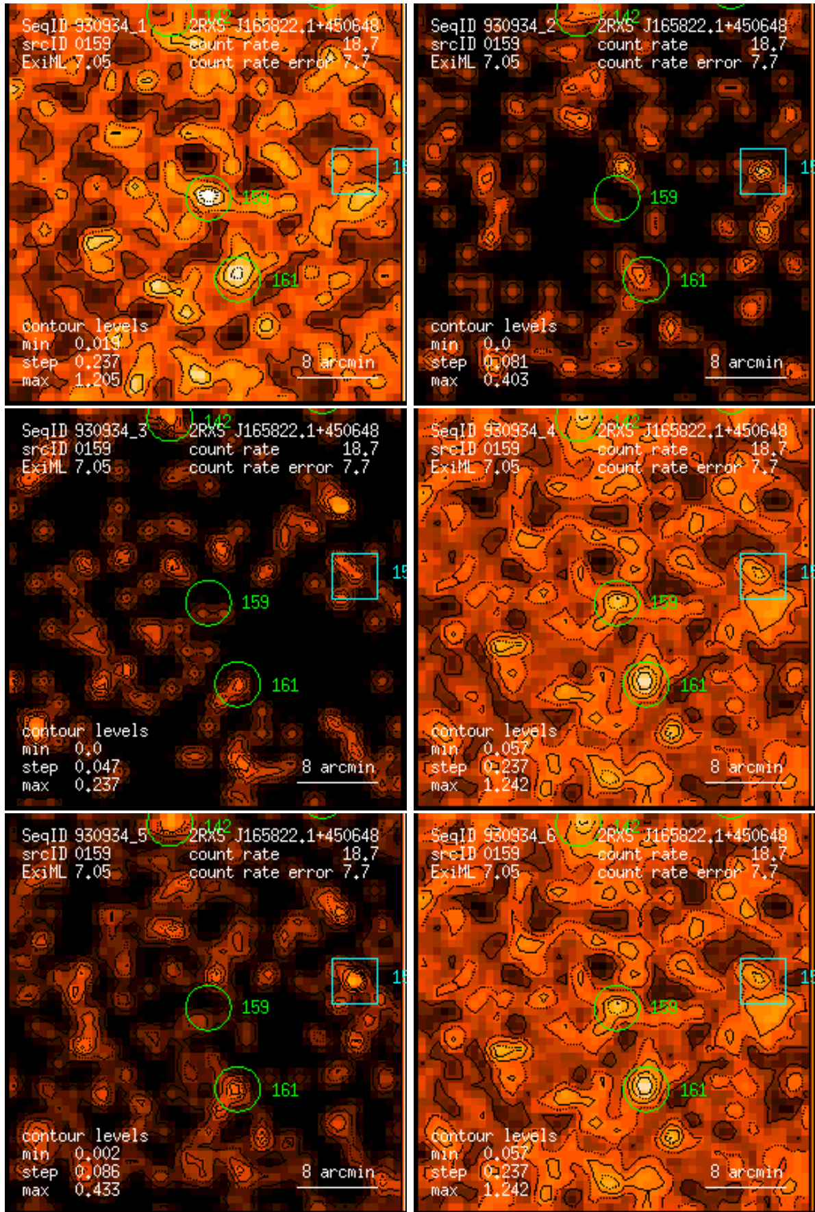
Figure 159: RASS 930934: detection 0159: band rate images, Gaussian filter: (1) PSPC channels 11 – 41, (2) 52 – 90, (3) 91 – 201, (4) 11 – 235, (5) 52 – 201, (6) 11 – 201. Broad band rates in counts/ks. Band rate contour levels in counts/ks/arcmin 2 .
