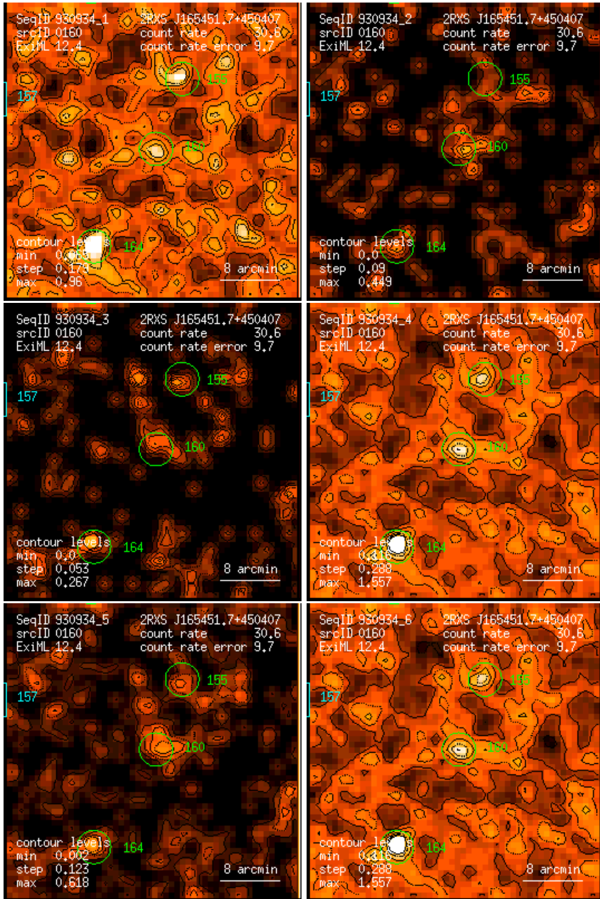
Figure 160: RASS 930934: detection 0160: band rate images, Gaussian filter: (1) PSPC channels 11 – 41, (2) 52 – 90, (3) 91 – 201, (4) 11 – 235, (5) 52 – 201, (6) 11 – 201. Broad band rates in counts/ks. Band rate contour levels in counts/ks/arcmin 2 .
