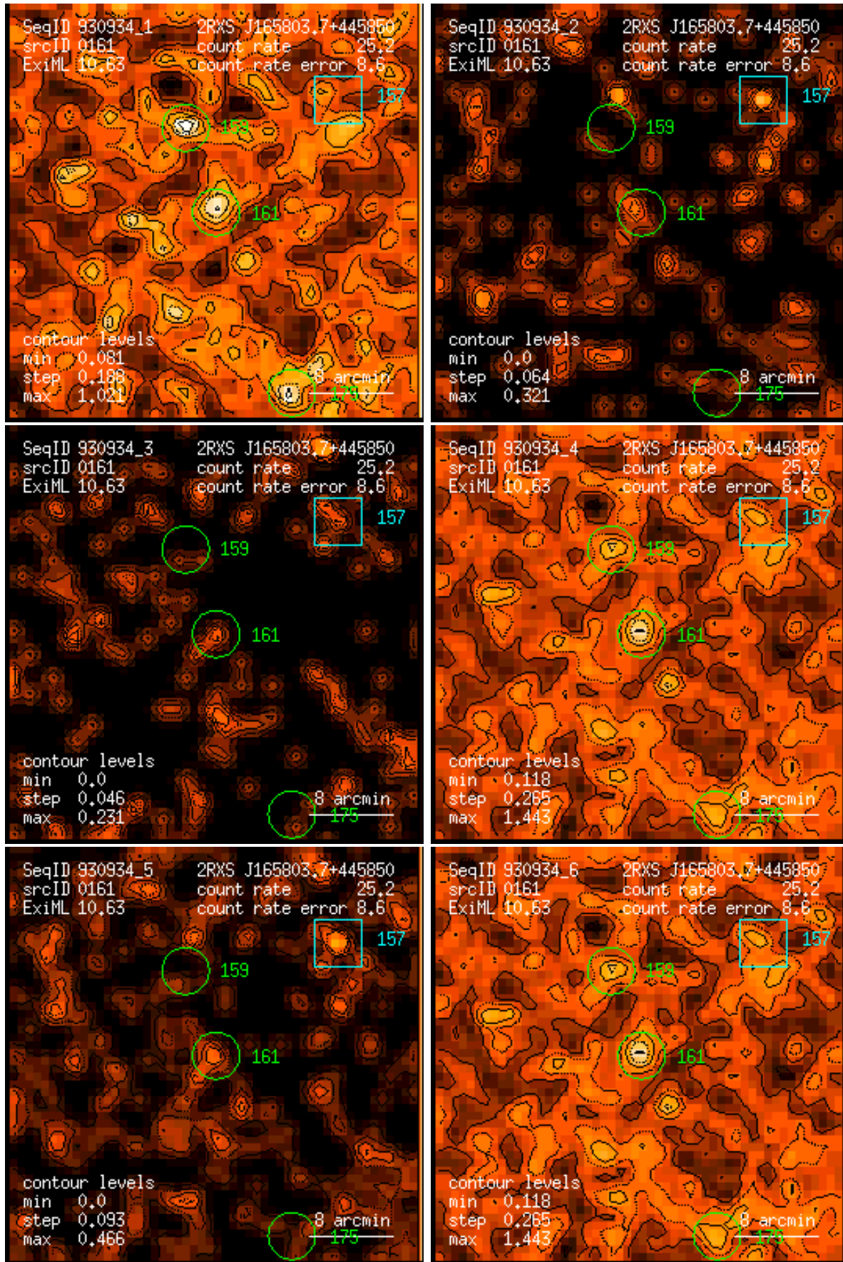
Figure 161: RASS 930934: detection 0161: band rate images, Gaussian filter: (1) PSPC channels 11 – 41, (2) 52 – 90, (3) 91 – 201, (4) 11 – 235, (5) 52 – 201, (6) 11 – 201. Broad band rates in counts/ks. Band rate contour levels in counts/ks/arcmin 2 .
