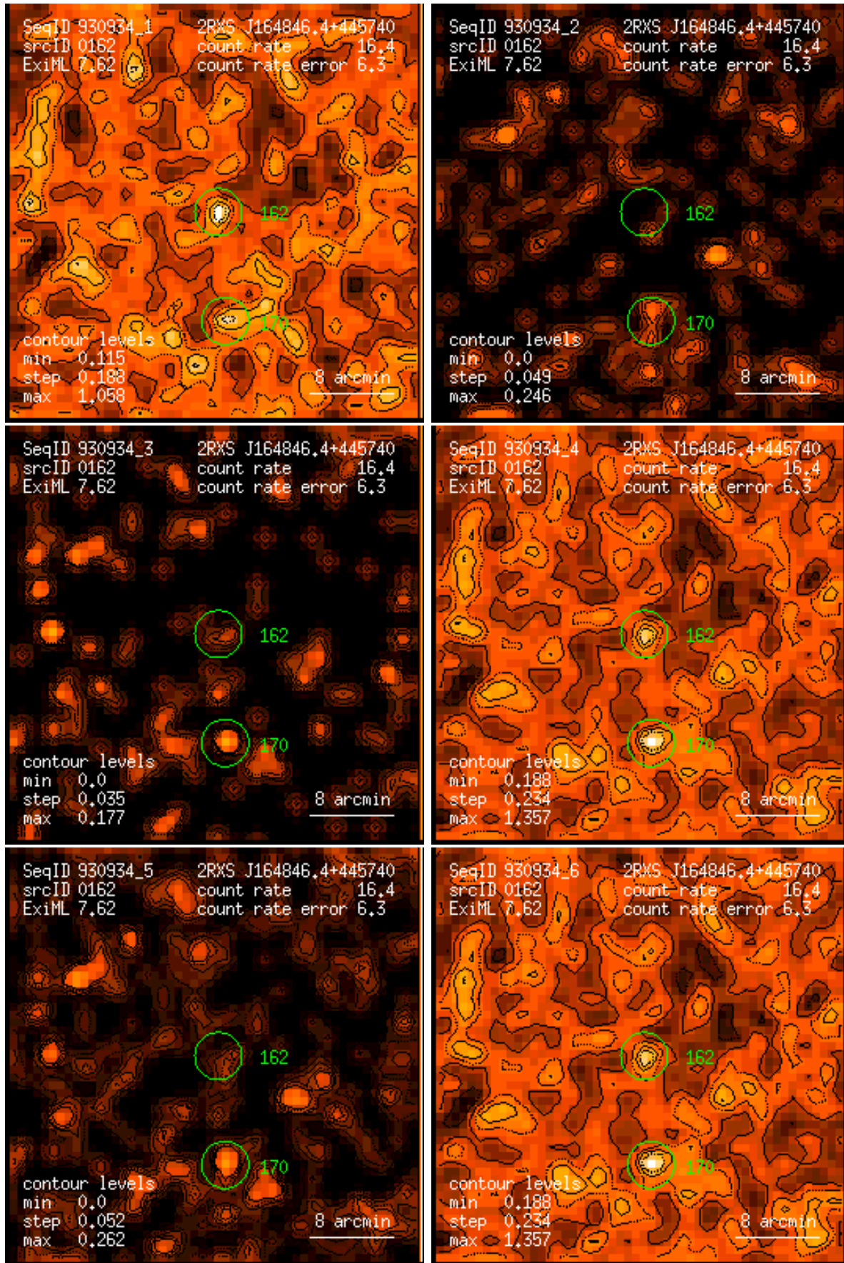
Figure 162: RASS 930934: detection 0162: band rate images, Gaussian filter: (1) PSPC channels 11 – 41, (2) 52 – 90, (3) 91 – 201, (4) 11 – 235, (5) 52 – 201, (6) 11 – 201. Broad band rates in counts/ks. Band rate contour levels in counts/ks/arcmin 2 .
