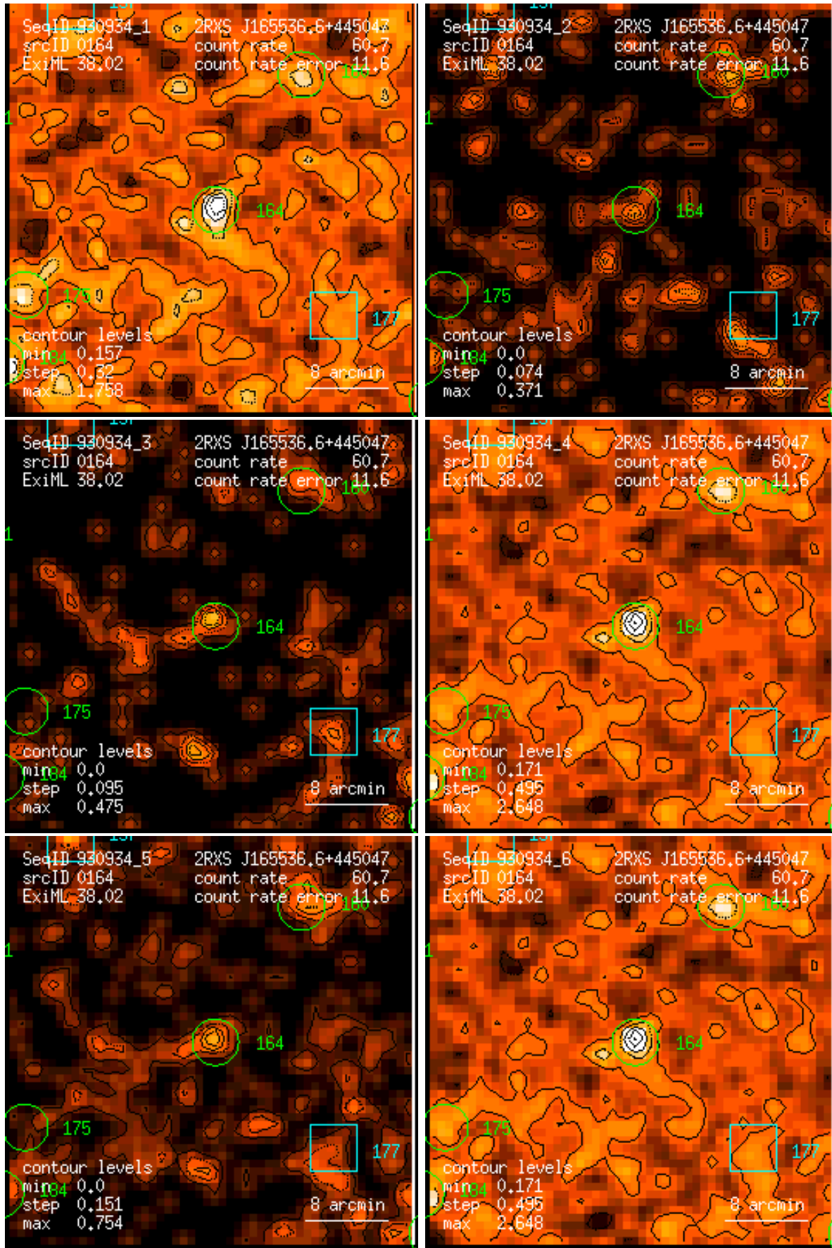
Figure 164: RASS 930934: detection 0164: band rate images, Gaussian filter: (1) PSPC channels 11 – 41, (2) 52 – 90, (3) 91 – 201, (4) 11 – 235, (5) 52 – 201, (6) 11 – 201. Broad band rates in counts/ks. Band rate contour levels in counts/ks/arcmin 2 .
