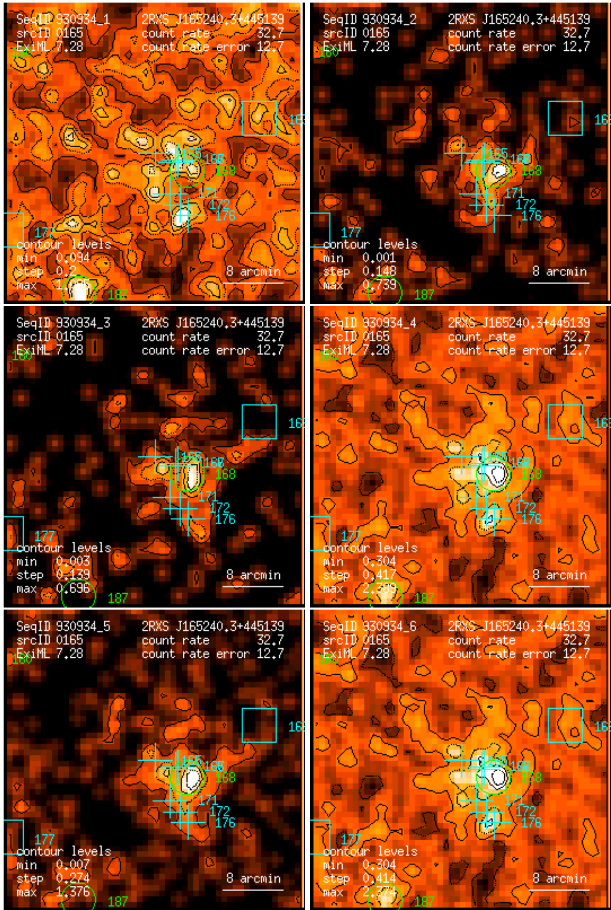
Figure 165: RASS 930934: detection 0165: band rate images, Gaussian filter: (1) PSPC channels 11 – 41, (2) 52 – 90, (3) 91 – 201, (4) 11 – 235, (5) 52 – 201, (6) 11 – 201. Broad band rates in counts/ks. Band rate contour levels in counts/ks/arcmin 2 .
