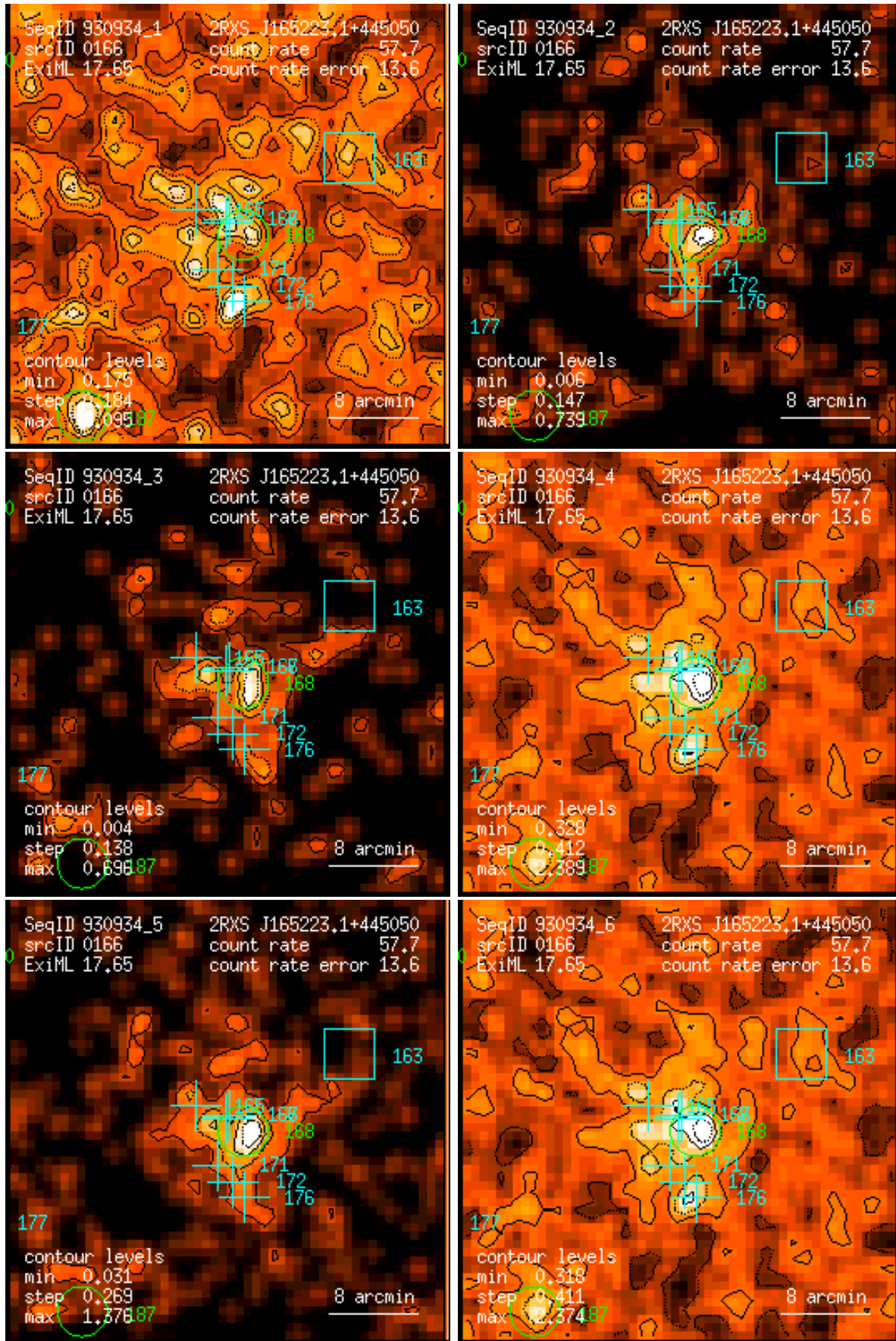
Figure 166: RASS 930934: detection 0166: band rate images, Gaussian filter: (1) PSPC channels 11 – 41, (2) 52 – 90, (3) 91 – 201, (4) 11 – 235, (5) 52 – 201, (6) 11 – 201. Broad band rates in counts/ks. Band rate contour levels in counts/ks/arcmin 2 .
