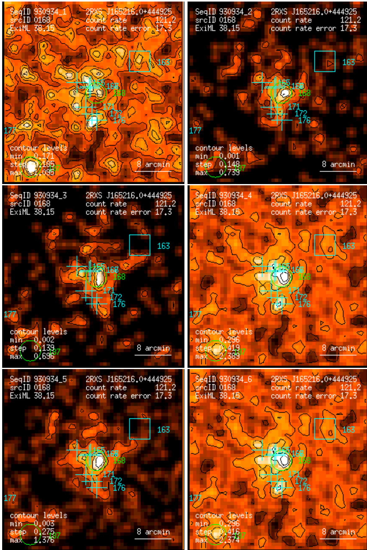
Figure 168: RASS 930934: detection 0168: band rate images, Gaussian filter: (1) PSPC channels 11 – 41, (2) 52 – 90, (3) 91 – 201, (4) 11 – 235, (5) 52 – 201, (6) 11 – 201. Broad band rates in counts/ks. Band rate contour levels in counts/ks/arcmin 2 .
