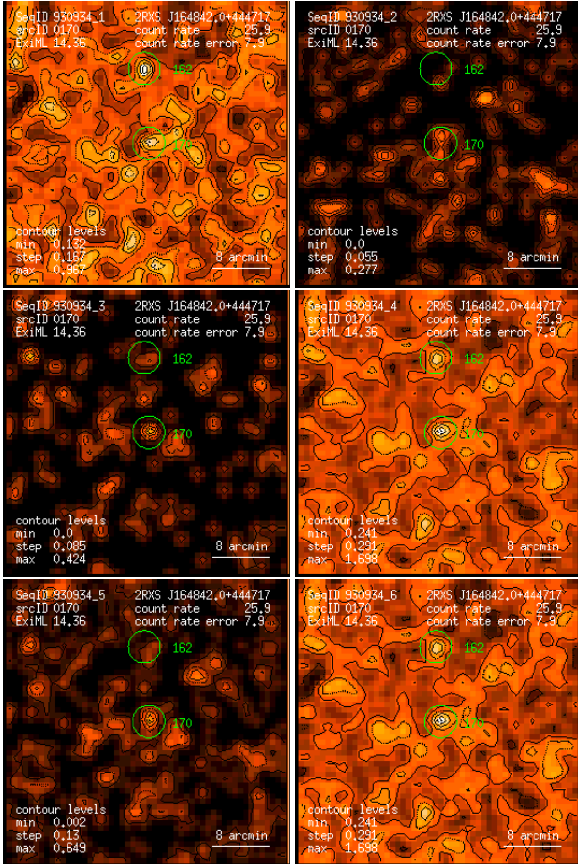
Figure 170: RASS 930934: detection 0170: band rate images, Gaussian filter: (1) PSPC channels 11 – 41, (2) 52 – 90, (3) 91 – 201, (4) 11 – 235, (5) 52 – 201, (6) 11 – 201. Broad band rates in counts/ks. Band rate contour levels in counts/ks/arcmin 2 .
