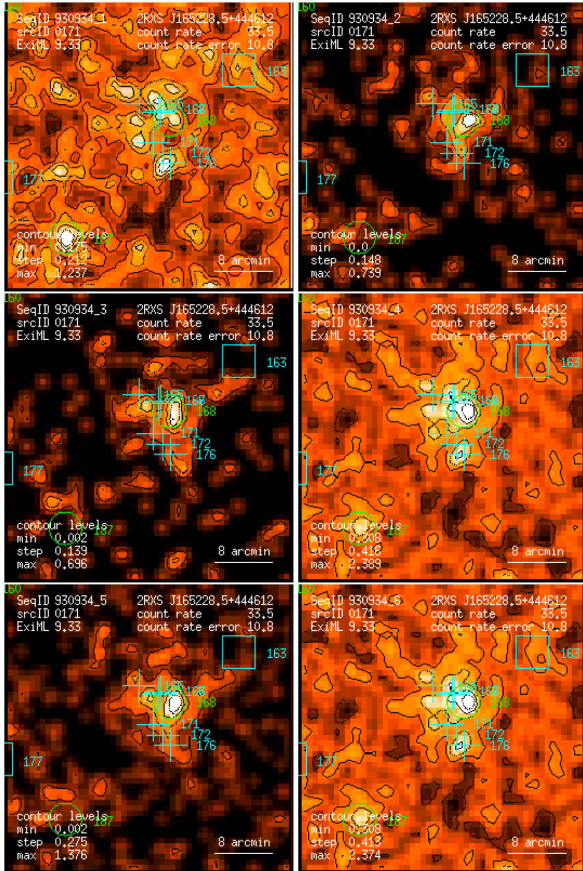
Figure 171: RASS 930934: detection 0171: band rate images, Gaussian filter: (1) PSPC channels 11 – 41, (2) 52 – 90, (3) 91 – 201, (4) 11 – 235, (5) 52 – 201, (6) 11 – 201. Broad band rates in counts/ks. Band rate contour levels in counts/ks/arcmin 2 .
