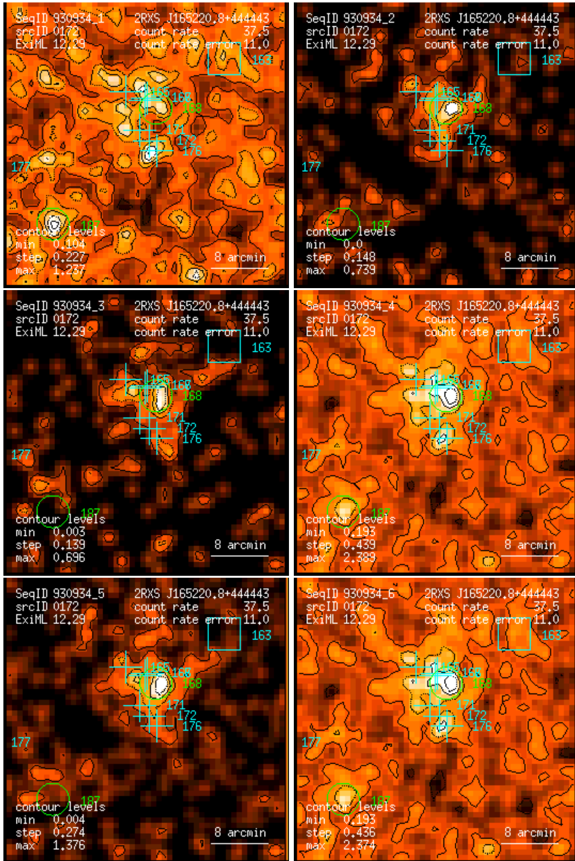
Figure 172: RASS 930934: detection 0172: band rate images, Gaussian filter: (1) PSPC channels 11 – 41, (2) 52 – 90, (3) 91 – 201, (4) 11 – 235, (5) 52 – 201, (6) 11 – 201. Broad band rates in counts/ks. Band rate contour levels in counts/ks/arcmin 2 .
