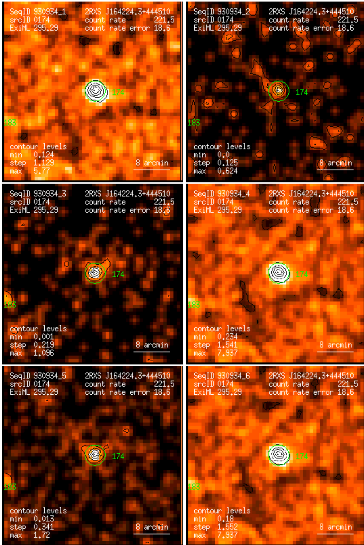
Figure 174: RASS 930934: detection 0174: band rate images, Gaussian filter: (1) PSPC channels 11 – 41, (2) 52 – 90, (3) 91 – 201, (4) 11 – 235, (5) 52 – 201, (6) 11 – 201. Broad band rates in counts/ks. Band rate contour levels in counts/ks/arcmin 2 .
