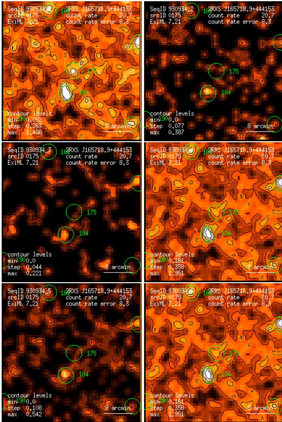
Figure 175: RASS 930934: detection 0175: band rate images, Gaussian filter: (1) PSPC channels 11 – 41, (2) 52 – 90, (3) 91 – 201, (4) 11 – 235, (5) 52 – 201, (6) 11 – 201. Broad band rates in counts/ks. Band rate contour levels in counts/ks/arcmin 2 .
