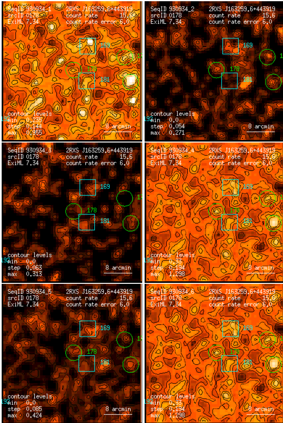
Figure 178: RASS 930934: detection 0178: band rate images, Gaussian filter: (1) PSPC channels 11 – 41, (2) 52 – 90, (3) 91 – 201, (4) 11 – 235, (5) 52 – 201, (6) 11 – 201. Broad band rates in counts/ks. Band rate contour levels in counts/ks/arcmin 2 .
