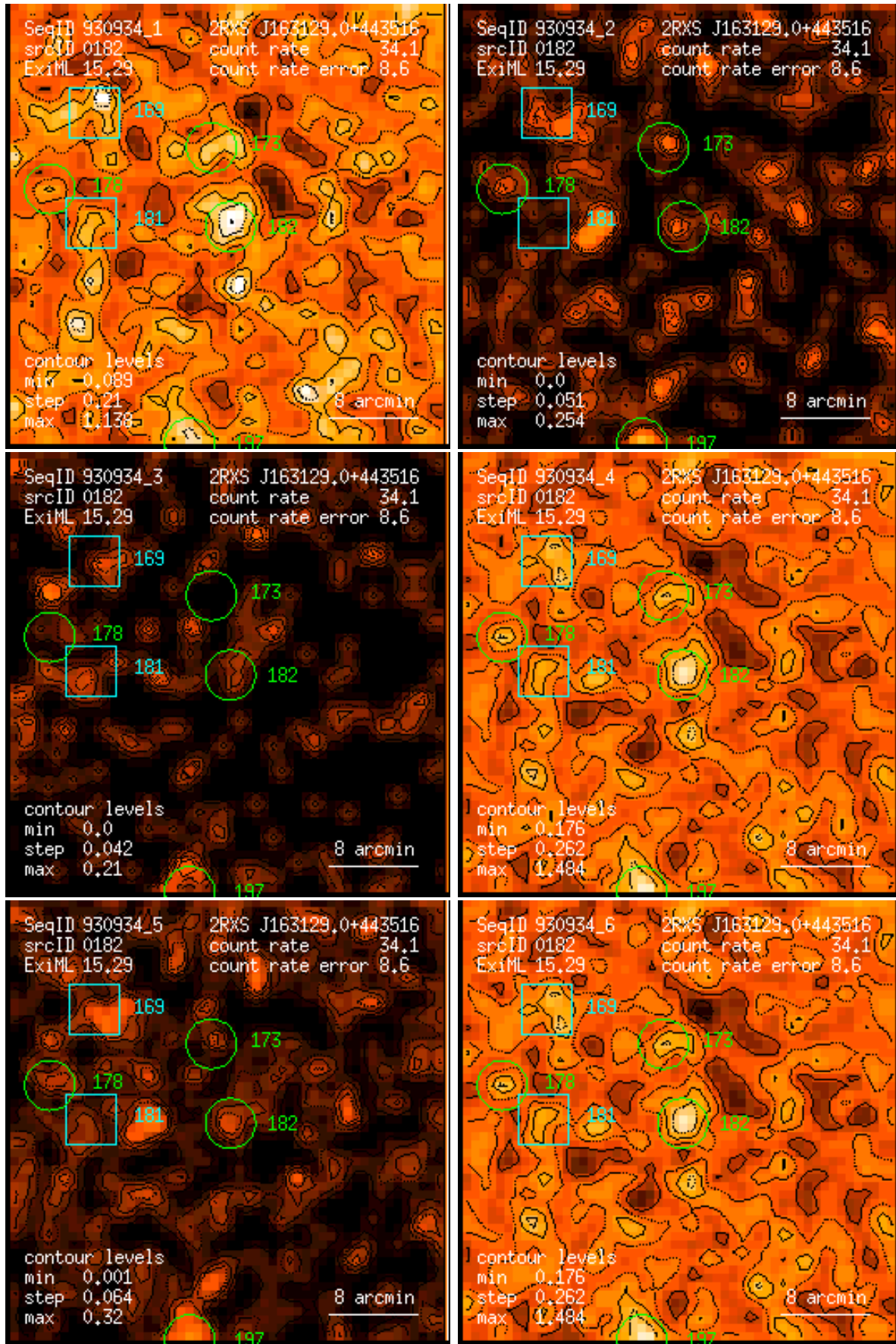
Figure 182: RASS 930934: detection 0182: band rate images, Gaussian filter: (1) PSPC channels 11 – 41, (2) 52 – 90, (3) 91 – 201, (4) 11 – 235, (5) 52 – 201, (6) 11 – 201. Broad band rates in counts/ks. Band rate contour levels in counts/ks/arcmin 2 .
