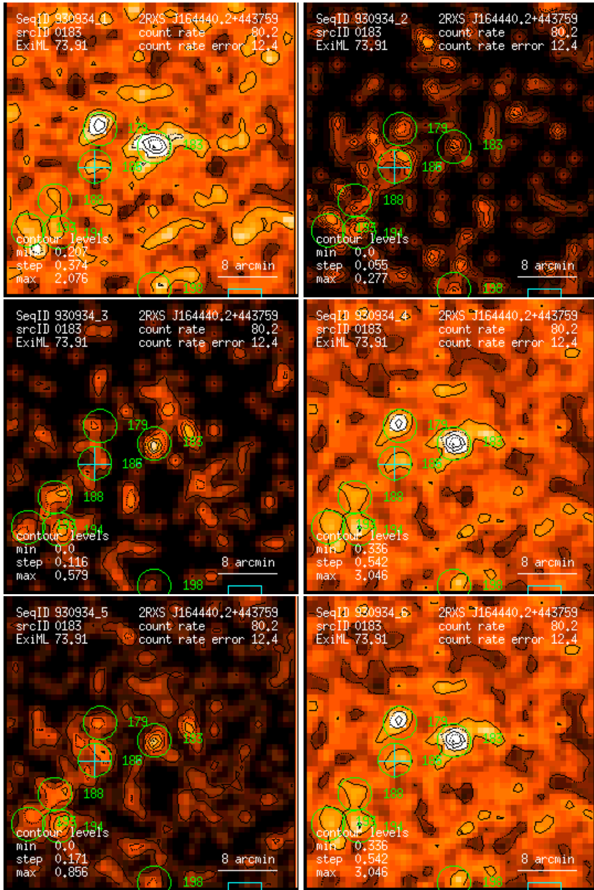
Figure 183: RASS 930934: detection 0183: band rate images, Gaussian filter: (1) PSPC channels 11 – 41, (2) 52 – 90, (3) 91 – 201, (4) 11 – 235, (5) 52 – 201, (6) 11 – 201. Broad band rates in counts/ks. Band rate contour levels in counts/ks/arcmin 2 .
