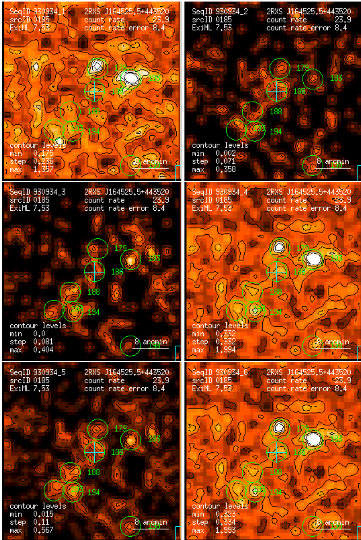
Figure 185: RASS 930934: detection 0185: band rate images, Gaussian filter: (1) PSPC channels 11 – 41, (2) 52 – 90, (3) 91 – 201, (4) 11 – 235, (5) 52 – 201, (6) 11 – 201. Broad band rates in counts/ks. Band rate contour levels in counts/ks/arcmin 2 .
