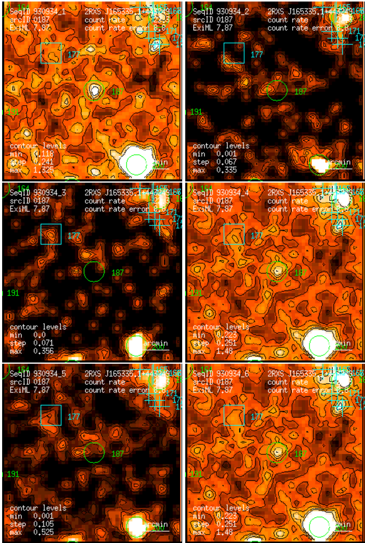
Figure 187: RASS 930934: detection 0187: band rate images, Gaussian filter: (1) PSPC channels 11 – 41, (2) 52 – 90, (3) 91 – 201, (4) 11 – 235, (5) 52 – 201, (6) 11 – 201. Broad band rates in counts/ks. Band rate contour levels in counts/ks/arcmin 2 .
