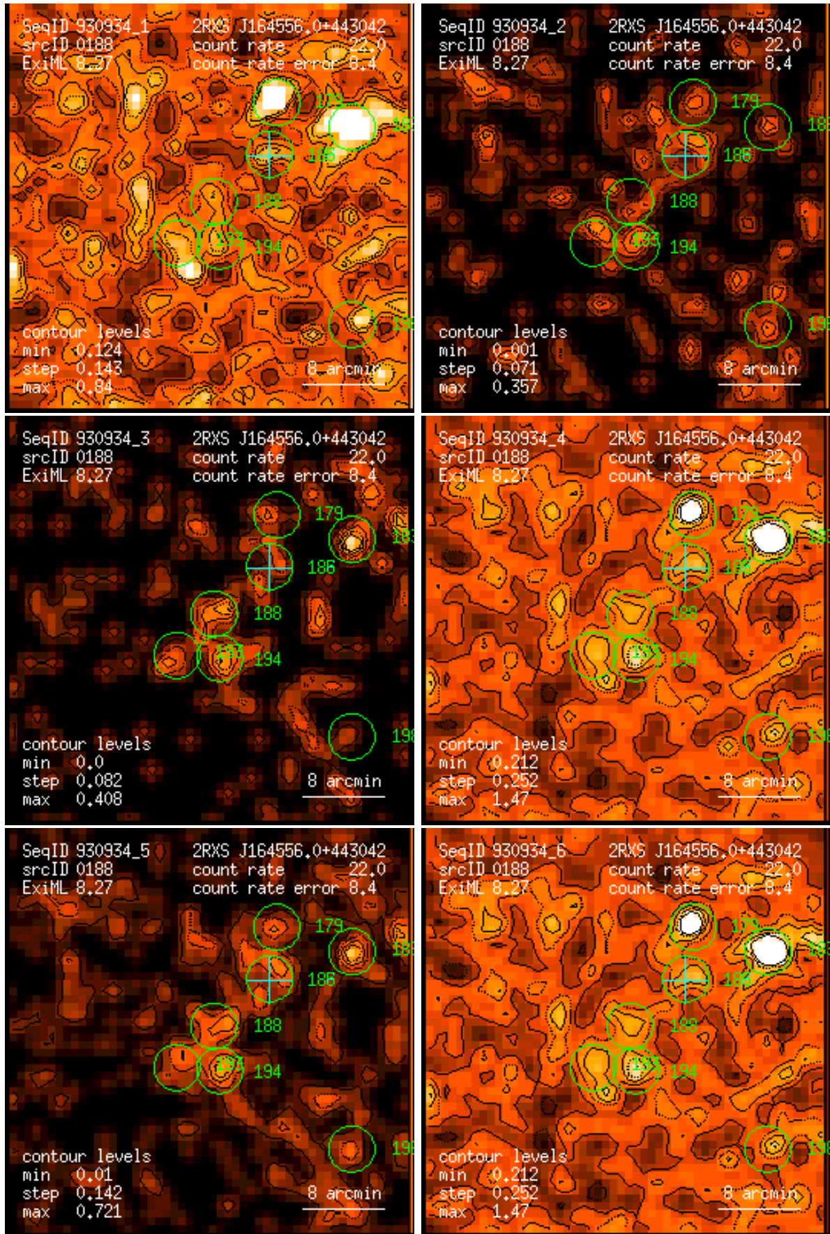
Figure 188: RASS 930934: detection 0188: band rate images, Gaussian filter: (1) PSPC channels 11 – 41, (2) 52 – 90, (3) 91 – 201, (4) 11 – 235, (5) 52 – 201, (6) 11 – 201. Broad band rates in counts/ks. Band rate contour levels in counts/ks/arcmin 2 .
