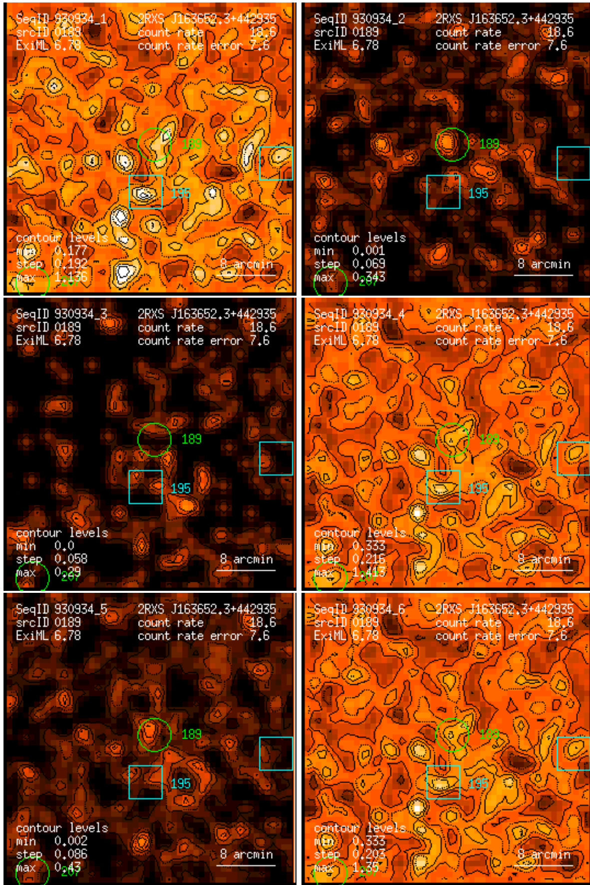
Figure 189: RASS 930934: detection 0189: band rate images, Gaussian filter: (1) PSPC channels 11 – 41, (2) 52 – 90, (3) 91 – 201, (4) 11 – 235, (5) 52 – 201, (6) 11 – 201. Broad band rates in counts/ks. Band rate contour levels in counts/ks/arcmin 2 .
