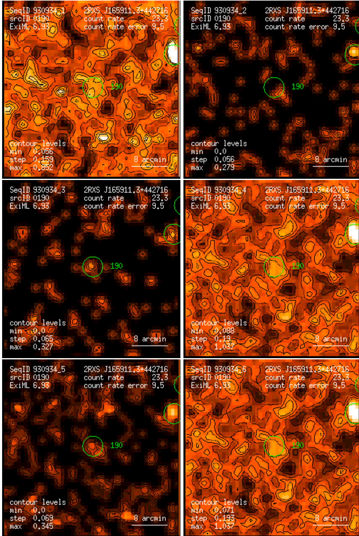
Figure 190: RASS 930934: detection 0190: band rate images, Gaussian filter: (1) PSPC channels 11 – 41, (2) 52 – 90, (3) 91 – 201, (4) 11 – 235, (5) 52 – 201, (6) 11 – 201. Broad band rates in counts/ks. Band rate contour levels in counts/ks/arcmin 2 .
