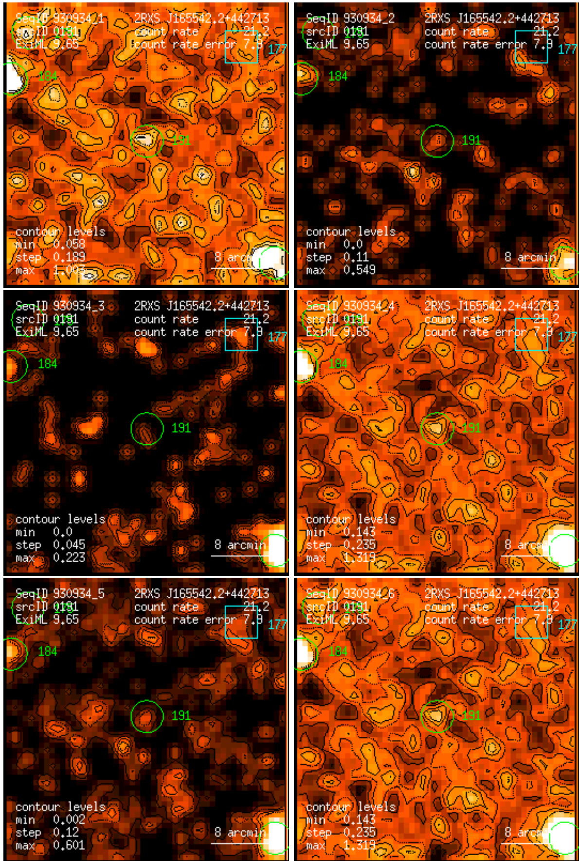
Figure 191: RASS 930934: detection 0191: band rate images, Gaussian filter: (1) PSPC channels 11 – 41, (2) 52 – 90, (3) 91 – 201, (4) 11 – 235, (5) 52 – 201, (6) 11 – 201. Broad band rates in counts/ks. Band rate contour levels in counts/ks/arcmin 2 .
