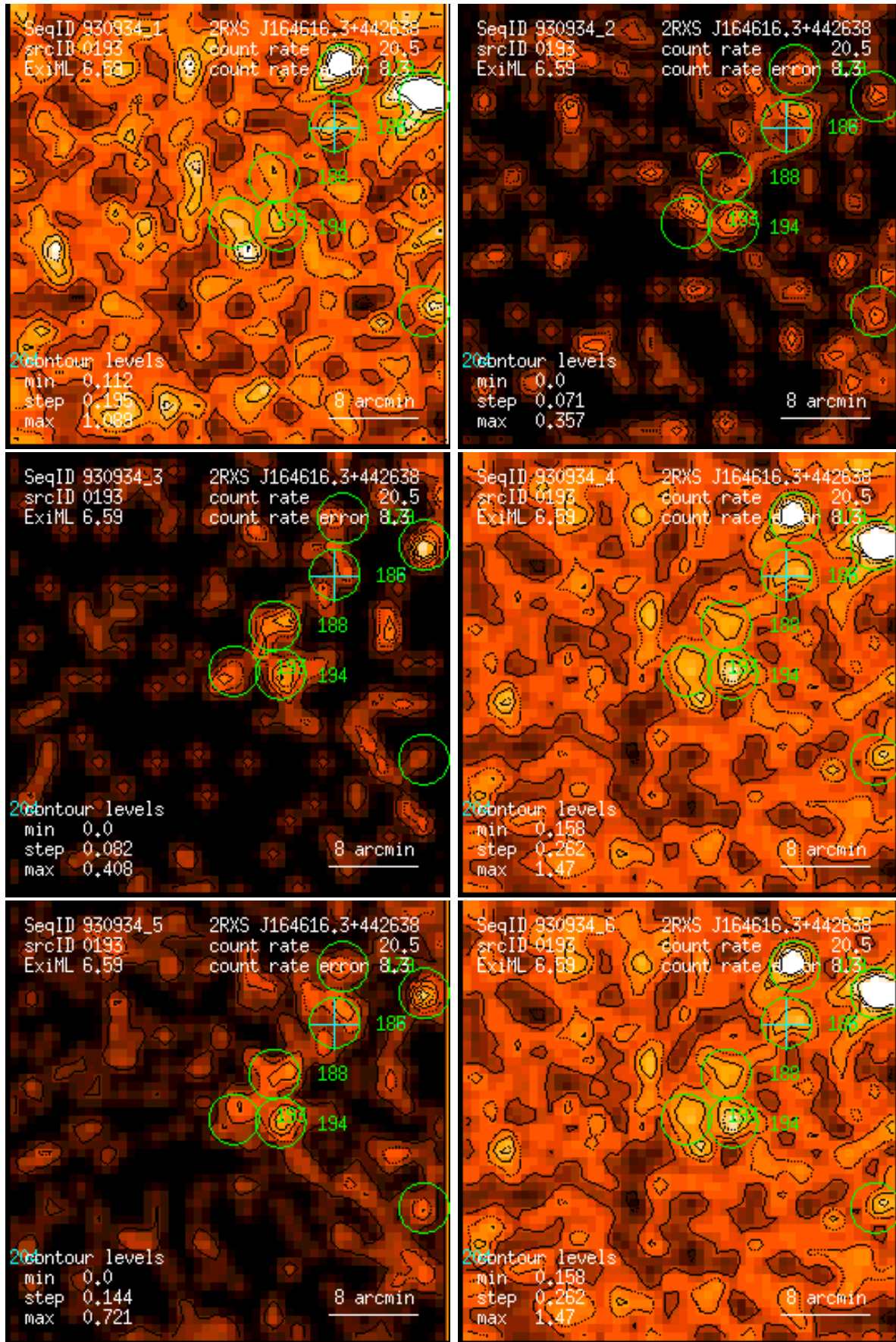
Figure 193: RASS 930934: detection 0193: band rate images, Gaussian filter: (1) PSPC channels 11 – 41, (2) 52 – 90, (3) 91 – 201, (4) 11 – 235, (5) 52 – 201, (6) 11 – 201. Broad band rates in counts/ks. Band rate contour levels in counts/ks/arcmin 2 .
