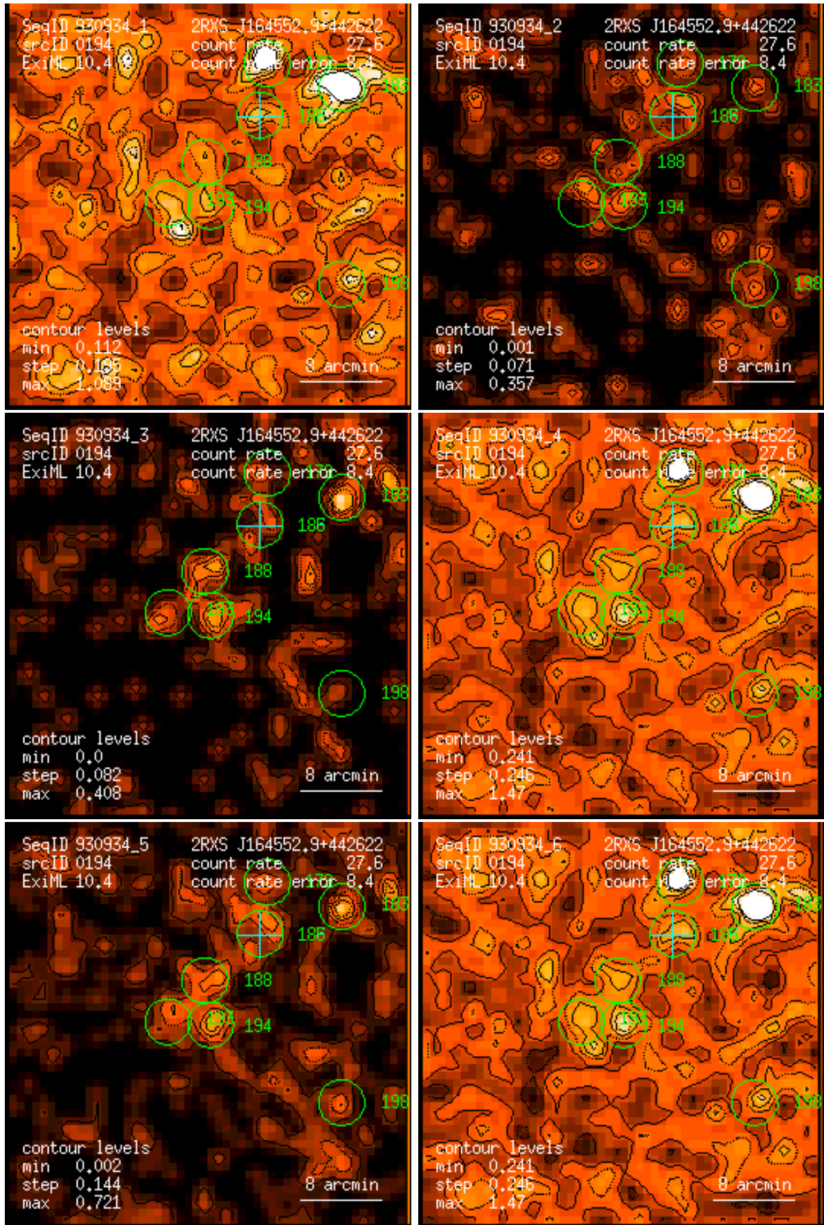
Figure 194: RASS 930934: detection 0194: band rate images, Gaussian filter: (1) PSPC channels 11 – 41, (2) 52 – 90, (3) 91 – 201, (4) 11 – 235, (5) 52 – 201, (6) 11 – 201. Broad band rates in counts/ks. Band rate contour levels in counts/ks/arcmin 2 .
