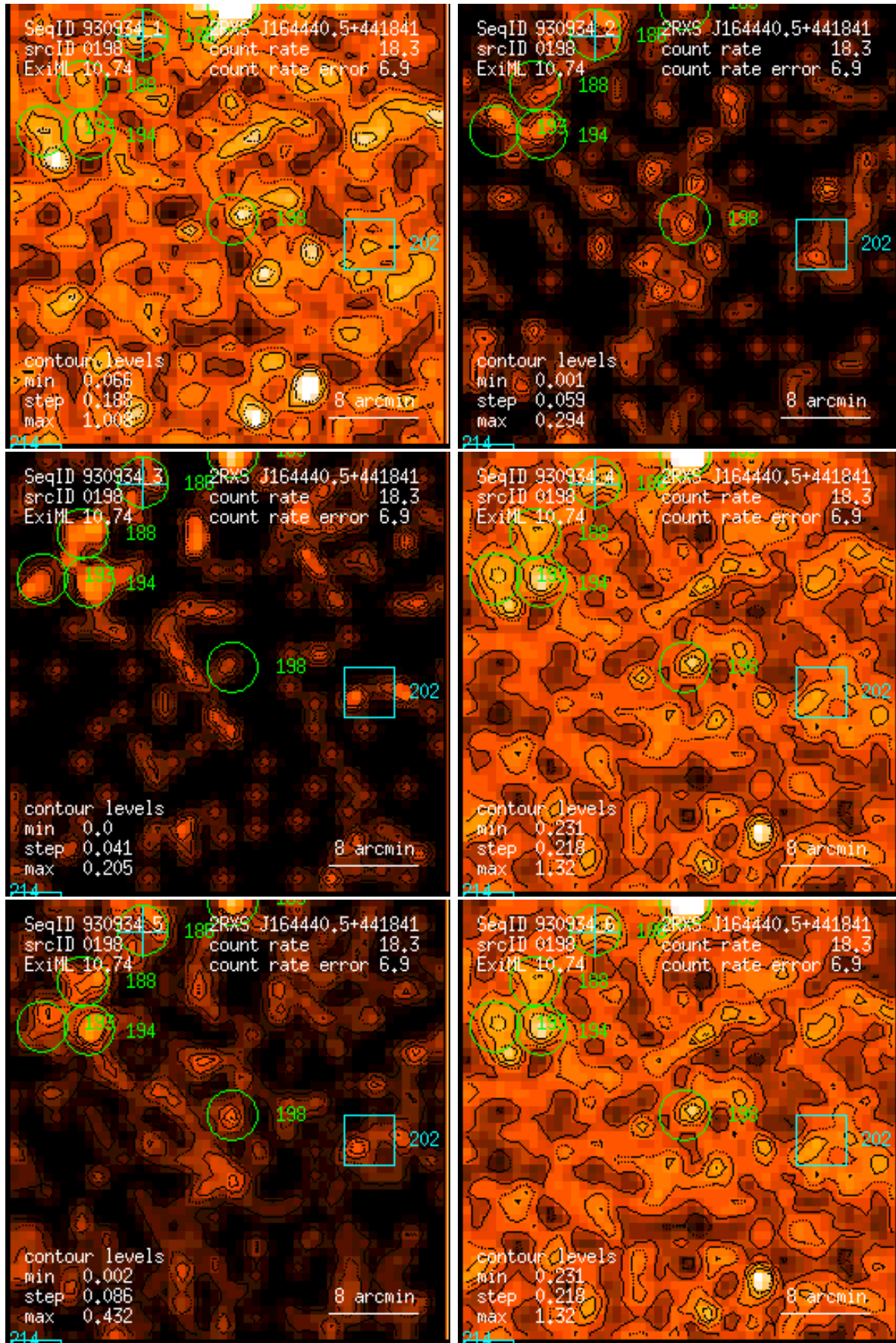
Figure 198: RASS 930934: detection 0198: band rate images, Gaussian filter: (1) PSPC channels 11 – 41, (2) 52 – 90, (3) 91 – 201, (4) 11 – 235, (5) 52 – 201, (6) 11 – 201. Broad band rates in counts/ks. Band rate contour levels in counts/ks/arcmin 2 .
