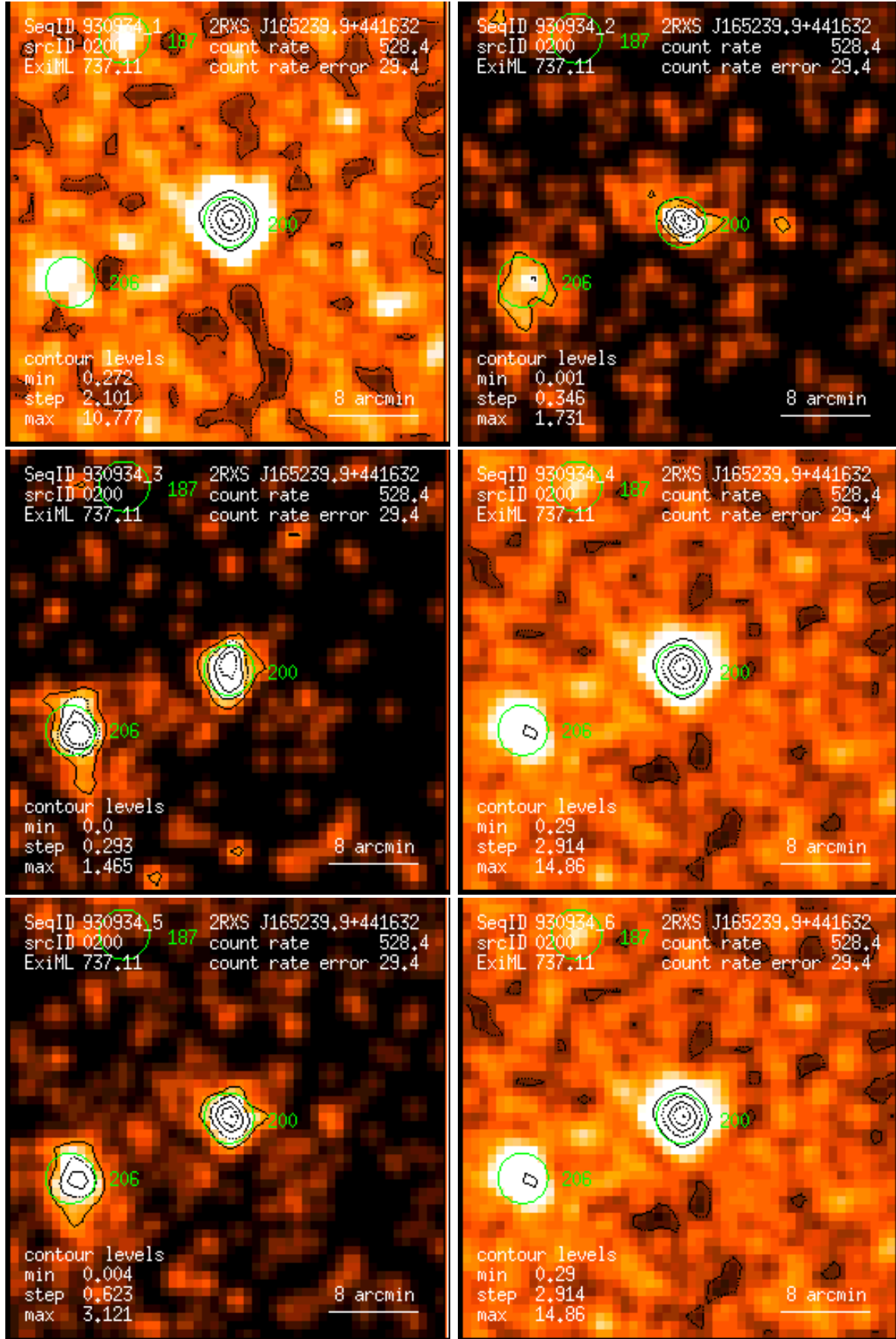
Figure 200: RASS 930934: detection 0200: band rate images, Gaussian filter: (1) PSPC channels 11 – 41, (2) 52 – 90, (3) 91 – 201, (4) 11 – 235, (5) 52 – 201, (6) 11 – 201. Broad band rates in counts/ks. Band rate contour levels in counts/ks/arcmin 2 .
