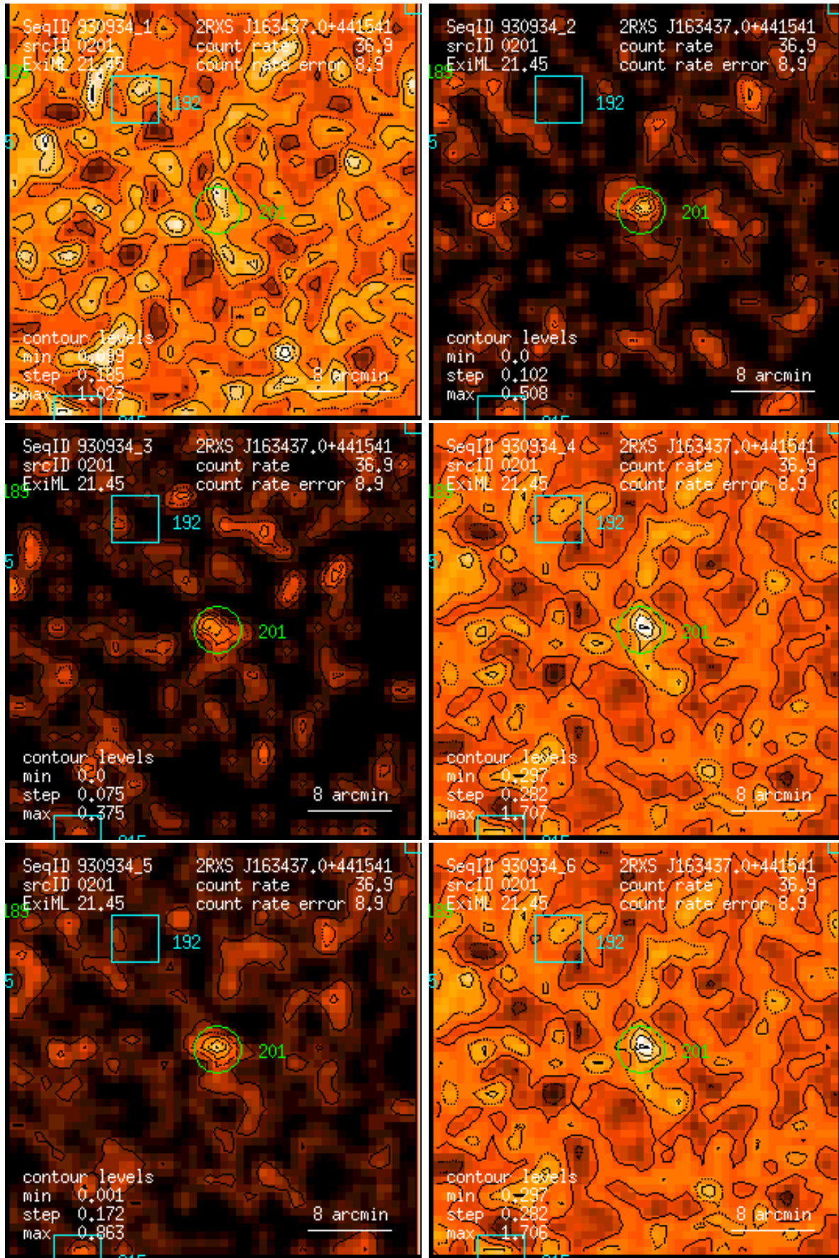
Figure 201: RASS 930934: detection 0201: band rate images, Gaussian filter: (1) PSPC channels 11 – 41, (2) 52 – 90, (3) 91 – 201, (4) 11 – 235, (5) 52 – 201, (6) 11 – 201. Broad band rates in counts/ks. Band rate contour levels in counts/ks/arcmin 2 .
