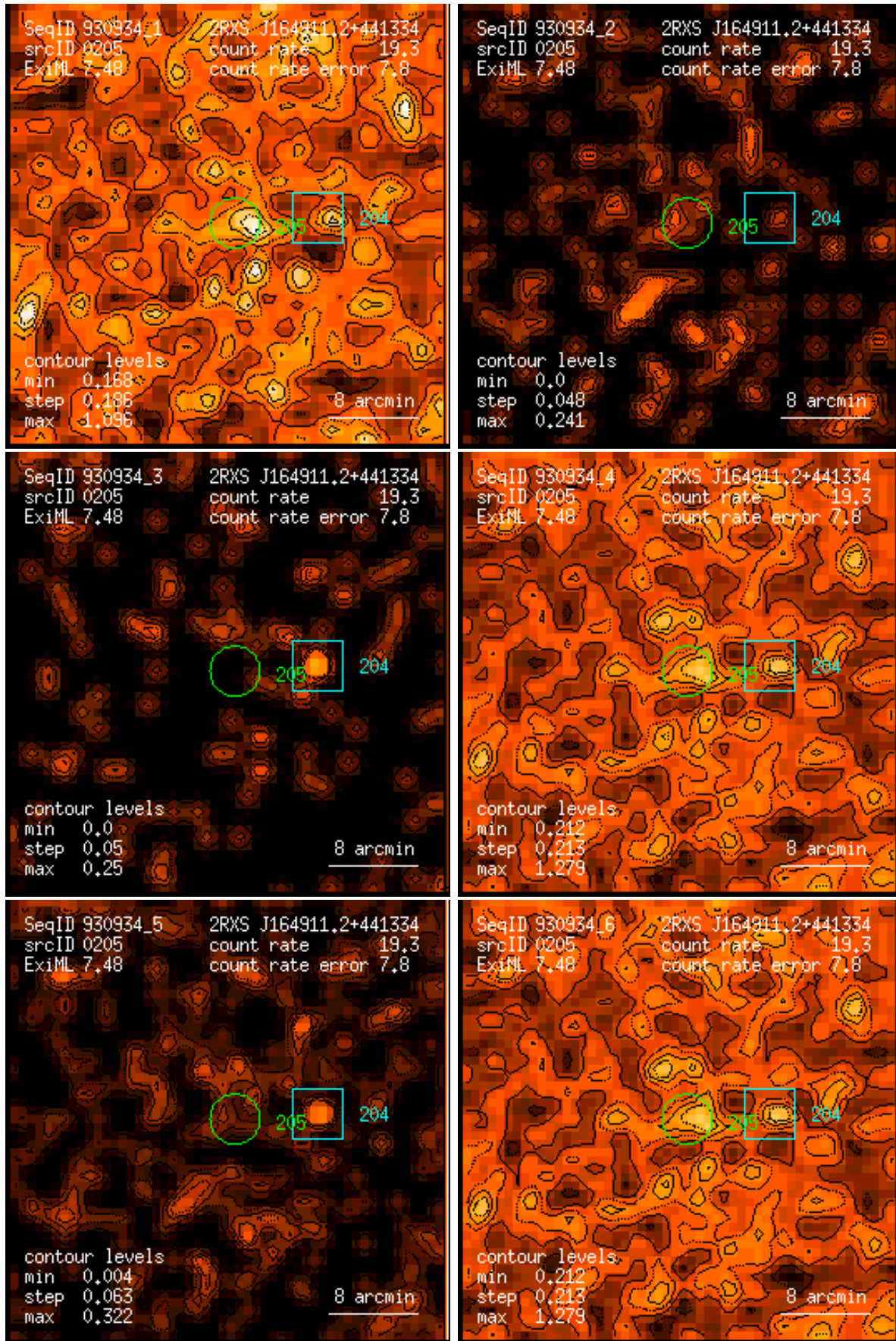
Figure 205: RASS 930934: detection 0205: band rate images, Gaussian filter: (1) PSPC channels 11 – 41, (2) 52 – 90, (3) 91 – 201, (4) 11 – 235, (5) 52 – 201, (6) 11 – 201. Broad band rates in counts/ks. Band rate contour levels in counts/ks/arcmin 2 .
