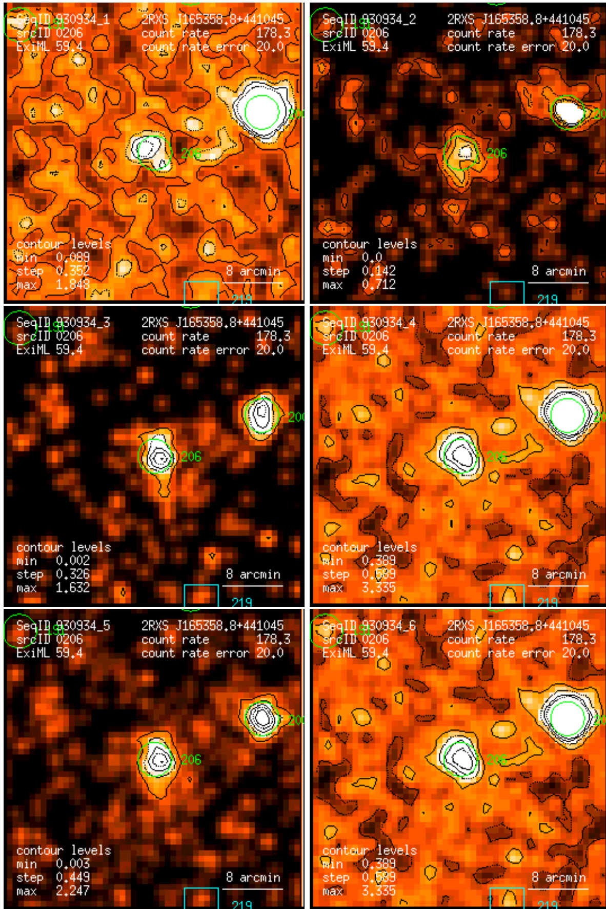
Figure 206: RASS 930934: detection 0206: band rate images, Gaussian filter: (1) PSPC channels 11 – 41, (2) 52 – 90, (3) 91 – 201, (4) 11 – 235, (5) 52 – 201, (6) 11 – 201. Broad band rates in counts/ks. Band rate contour levels in counts/ks/arcmin 2 .
