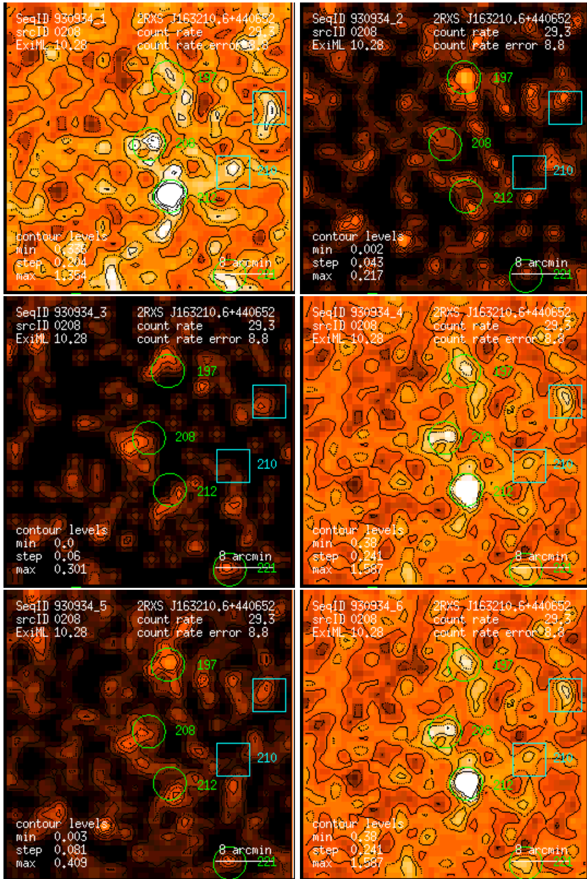
Figure 208: RASS 930934: detection 0208: band rate images, Gaussian filter: (1) PSPC channels 11 – 41, (2) 52 – 90, (3) 91 – 201, (4) 11 – 235, (5) 52 – 201, (6) 11 – 201. Broad band rates in counts/ks. Band rate contour levels in counts/ks/arcmin 2 .
