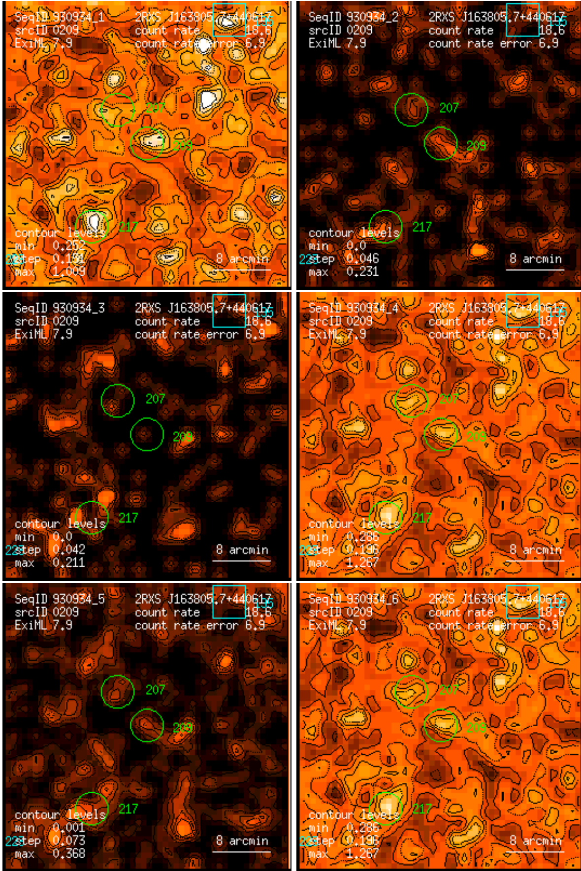
Figure 209: RASS 930934: detection 0209: band rate images, Gaussian filter: (1) PSPC channels 11 – 41, (2) 52 – 90, (3) 91 – 201, (4) 11 – 235, (5) 52 – 201, (6) 11 – 201. Broad band rates in counts/ks. Band rate contour levels in counts/ks/arcmin 2 .
