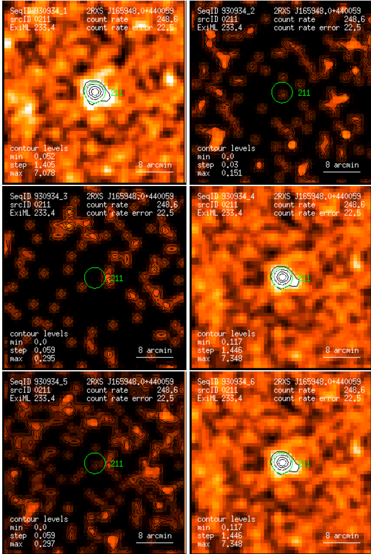
Figure 211: RASS 930934: detection 0211: band rate images, Gaussian filter: (1) PSPPC channels 11 – 41, (2) 52 – 90, (3) 91 – 201, (4) 11 – 235, (5) 52 – 201, (6) 11 – 201. Broad band rates in counts/ks. Band rate contour levels in counts/ks/arcmin 2 .
