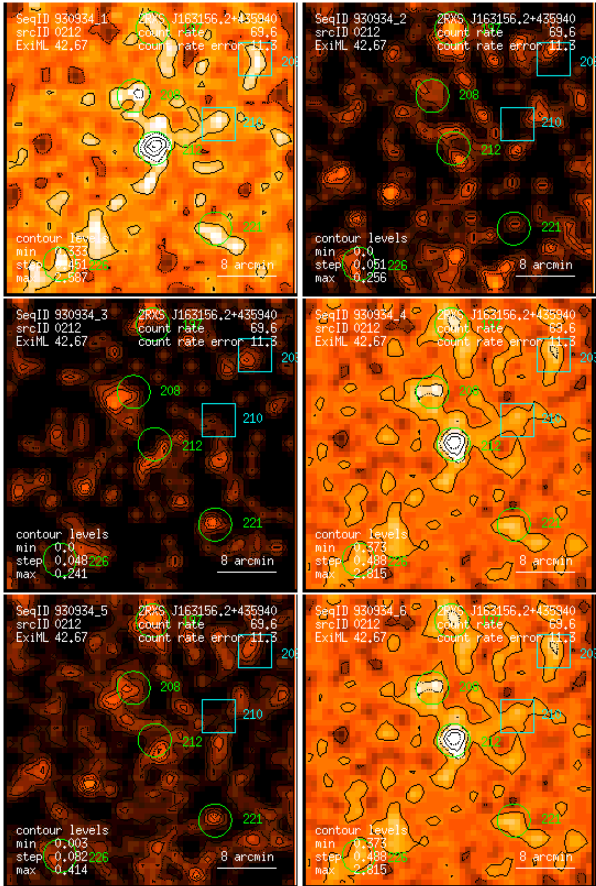
Figure 212: RASS 930934: detection 0212: band rate images, Gaussian filter: (1) PSPC channels 11 – 41, (2) 52 – 90, (3) 91 – 201, (4) 11 – 235, (5) 52 – 201, (6) 11 – 201. Broad band rates in counts/ks. Band rate contour levels in counts/ks/arcmin 2 .
