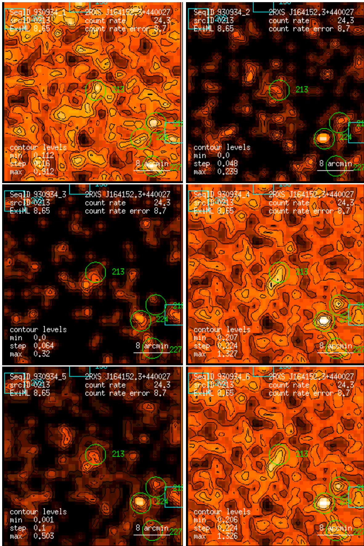
Figure 213: RASS 930934: detection 0213: band rate images, Gaussian filter: (1) PSPC channels 11 – 41, (2) 52 – 90, (3) 91 – 201, (4) 11 – 235, (5) 52 – 201, (6) 11 – 201. Broad band rates in counts/ks. Band rate contour levels in counts/ks/arcmin 2 .
