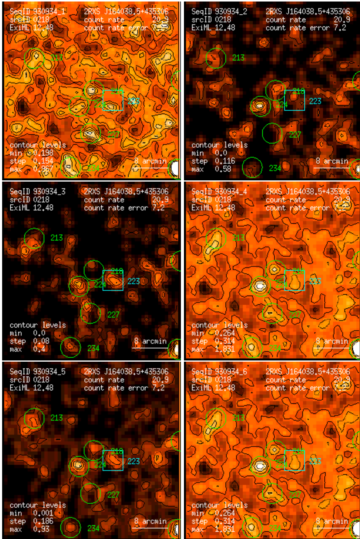
Figure 218: RASS 930934: detection 0218: band rate images, Gaussian filter: (1) PSPC channels 11 – 41, (2) 52 – 90, (3) 91 – 201, (4) 11 – 235, (5) 52 – 201, (6) 11 – 201. Broad band rates in counts/ks. Band rate contour levels in counts/ks/arcmin 2 .
