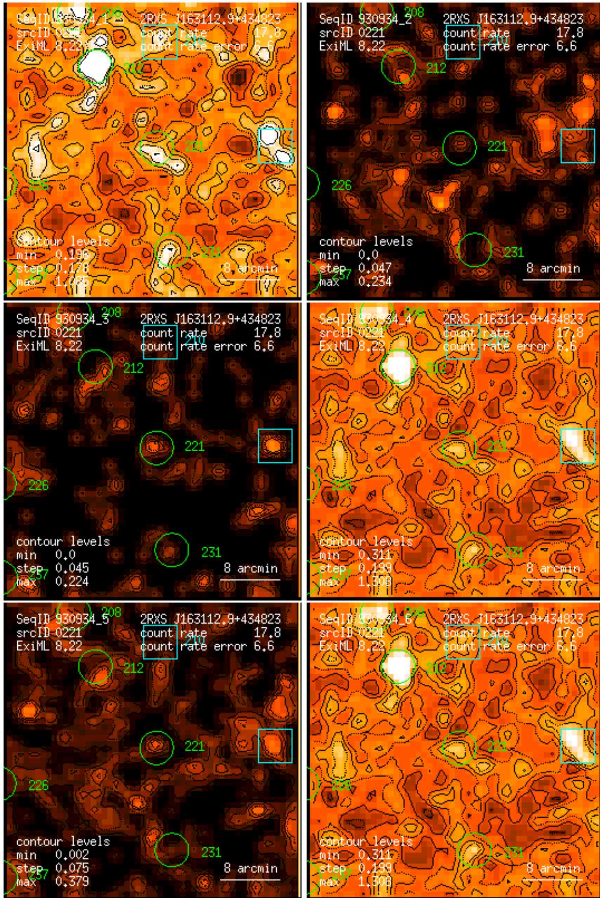
Figure 221: RASS 930934: detection 0221: band rate images, Gaussian filter: (1) PSPC channels 11 – 41, (2) 52 – 90, (3) 91 – 201, (4) 11 – 235, (5) 52 – 201, (6) 11 – 201. Broad band rates in counts/ks. Band rate contour levels in counts/ks/arcmin 2 .
