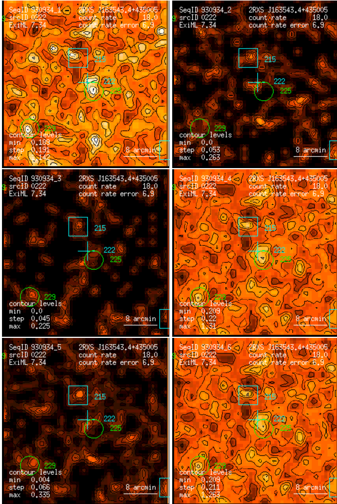
Figure 222: RASS 930934: detection 0222: band rate images, Gaussian filter: (1) PSPC channels 11 – 41, (2) 52 – 90, (3) 91 – 201, (4) 11 – 235, (5) 52 – 201, (6) 11 – 201. Broad band rates in counts/ks. Band rate contour levels in counts/ks/arcmin 2 .
