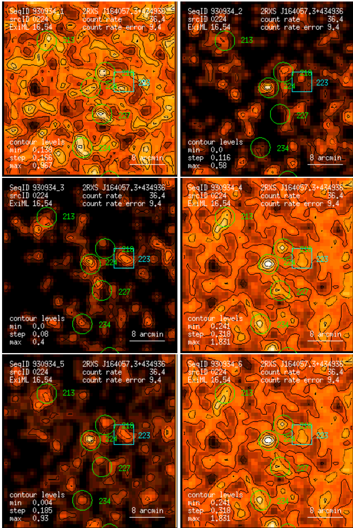
Figure 224: RASS 930934: detection 0224: band rate images, Gaussian filter: (1) PSPC channels 11 – 41, (2) 52 – 90, (3) 91 – 201, (4) 11 – 235, (5) 52 – 201, (6) 11 – 201. Broad band rates in counts/ks. Band rate contour levels in counts/ks/arcmin 2 .
