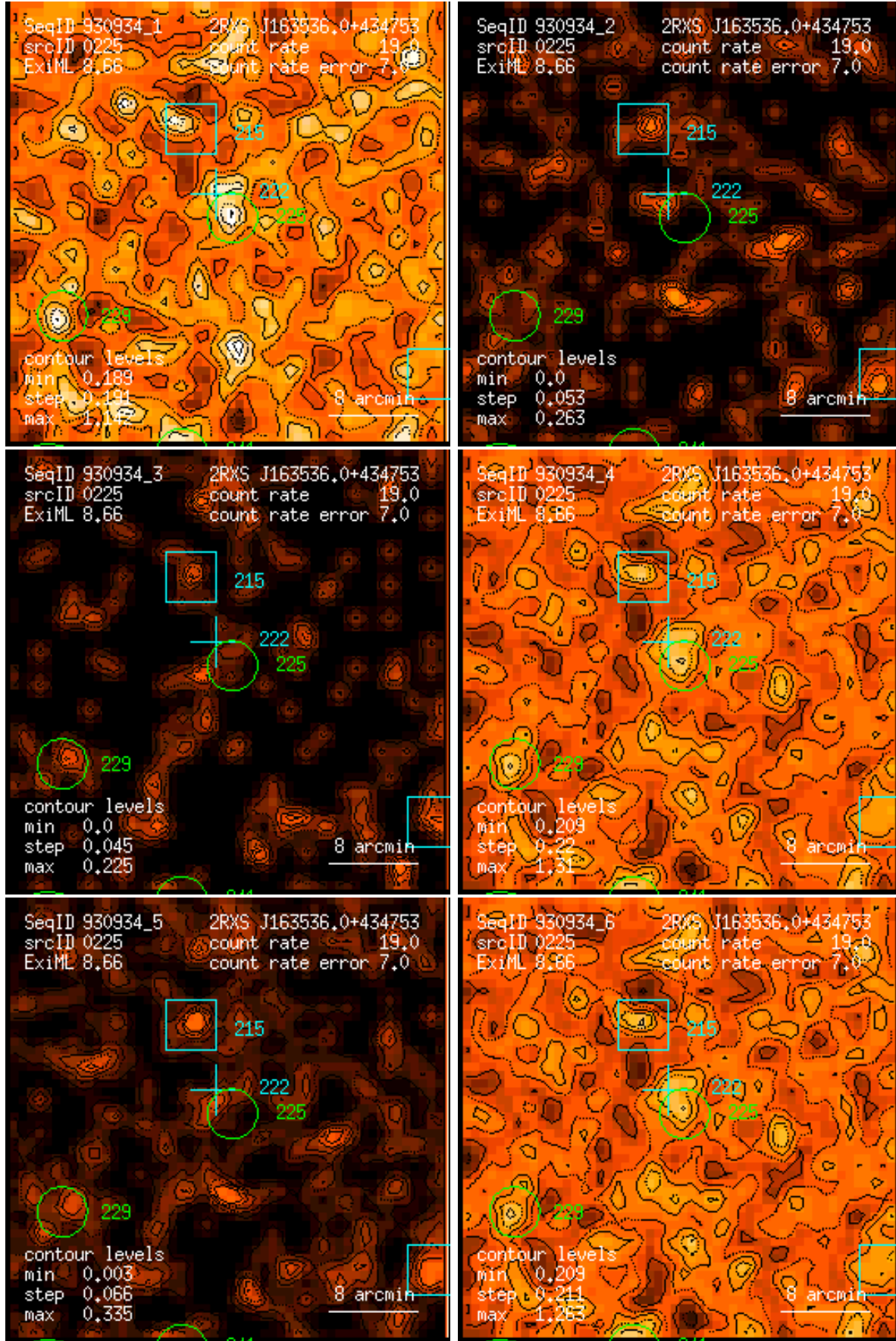
Figure 225: RASS 930934: detection 0225: band rate images, Gaussian filter: (1) PSPC channels 11 – 41, (2) 52 – 90, (3) 91 – 201, (4) 11 – 235, (5) 52 – 201, (6) 11 – 201. Broad band rates in counts/ks. Band rate contour levels in counts/ks/arcmin 2 .
