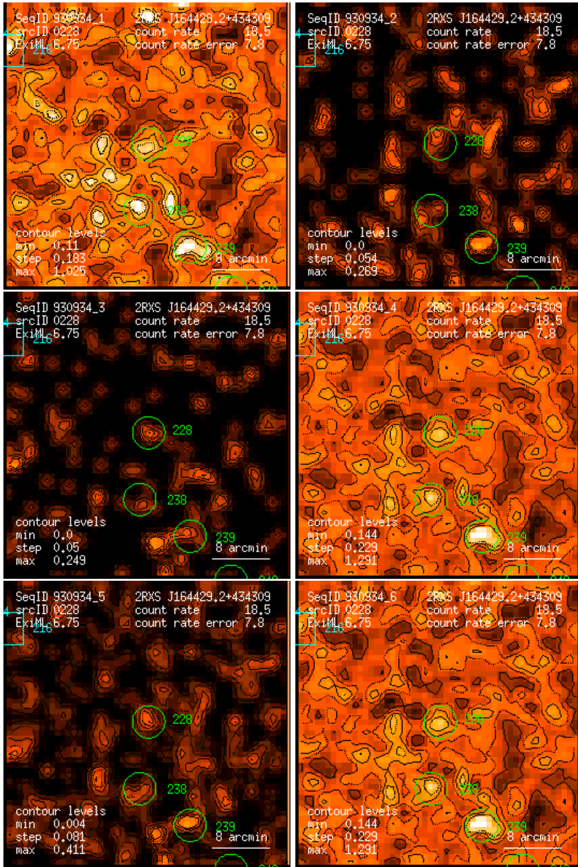
Figure 228: RASS 930934: detection 0228: band rate images, Gaussian filter: (1) PSPC channels 11 – 41, (2) 52 – 90, (3) 91 – 201, (4) 11 – 235, (5) 52 – 201, (6) 11 – 201. Broad band rates in counts/ks. Band rate contour levels in counts/ks/arcmin 2 .
