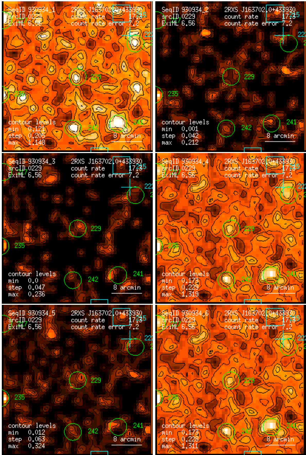
Figure 229: RASS 930934: detection 0229: band rate images, Gaussian filter: (1) PSPC channels 11 – 41, (2) 52 – 90, (3) 91 – 201, (4) 11 – 235, (5) 52 – 201, (6) 11 – 201. Broad band rates in counts/ks. Band rate contour levels in counts/ks/arcmin 2 .
