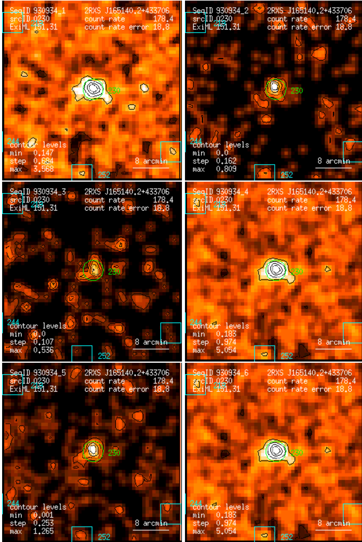
Figure 230: RASS 930934: detection 0230: band rate images, Gaussian filter: (1) PSPC channels 11 – 41, (2) 52 – 90, (3) 91 – 201, (4) 11 – 235, (5) 52 – 201, (6) 11 – 201. Broad band rates in counts/ks. Band rate contour levels in counts/ks/arcmin 2 .
