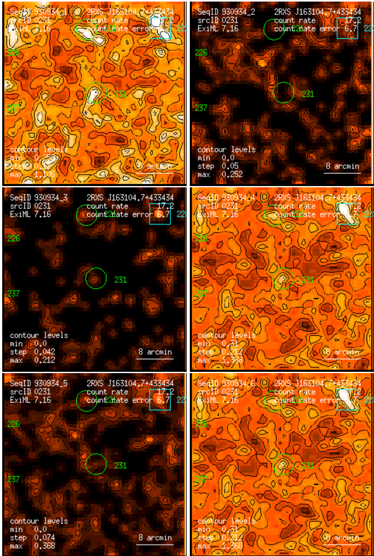
Figure 231: RASS 930934: detection 0231: band rate images, Gaussian filter: (1) PSPC channels 11 – 41, (2) 52 – 90, (3) 91 – 201, (4) 11 – 235, (5) 52 – 201, (6) 11 – 201. Broad band rates in counts/ks. Band rate contour levels in counts/ks/arcmin 2 .
