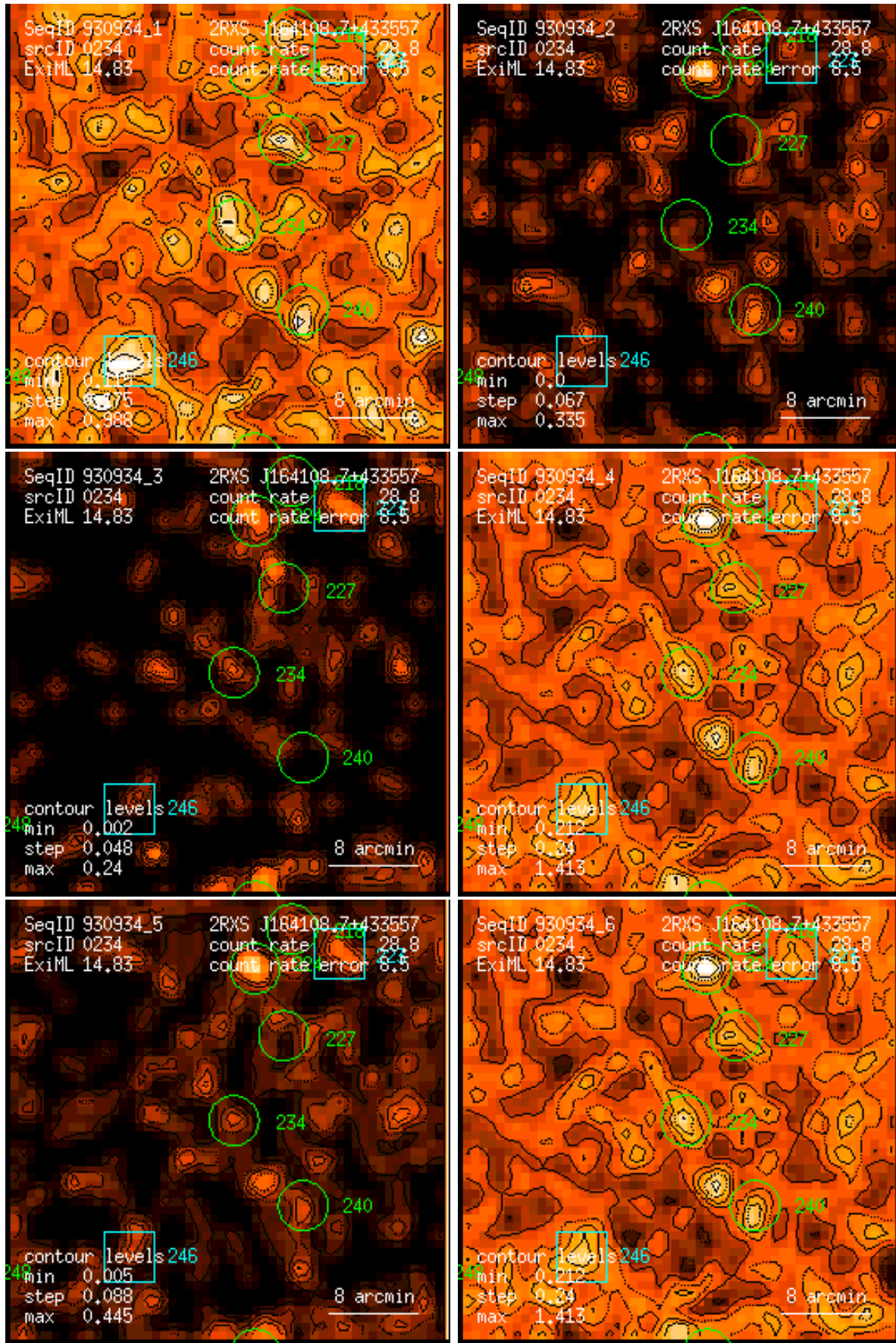
Figure 234: RASS 930934: detection 0234: band rate images, Gaussian filter: (1) PSPC channels 11 – 41, (2) 52 – 90, (3) 91 – 201, (4) 11 – 235, (5) 52 – 201, (6) 11 – 201. Broad band rates in counts/ks. Band rate contour levels in counts/ks/arcmin 2 .
