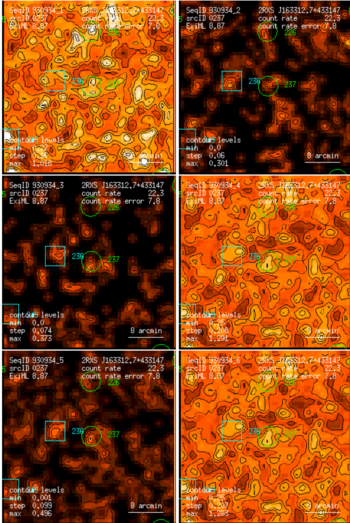
Figure 237: RASS 930934: detection 0237: band rate images, Gaussian filter: (1) PSPC channels 11 – 41, (2) 52 – 90, (3) 91 – 201, (4) 11 – 235, (5) 52 – 201, (6) 11 – 201. Broad band rates in counts/ks. Band rate contour levels in counts/ks/arcmin 2 .
