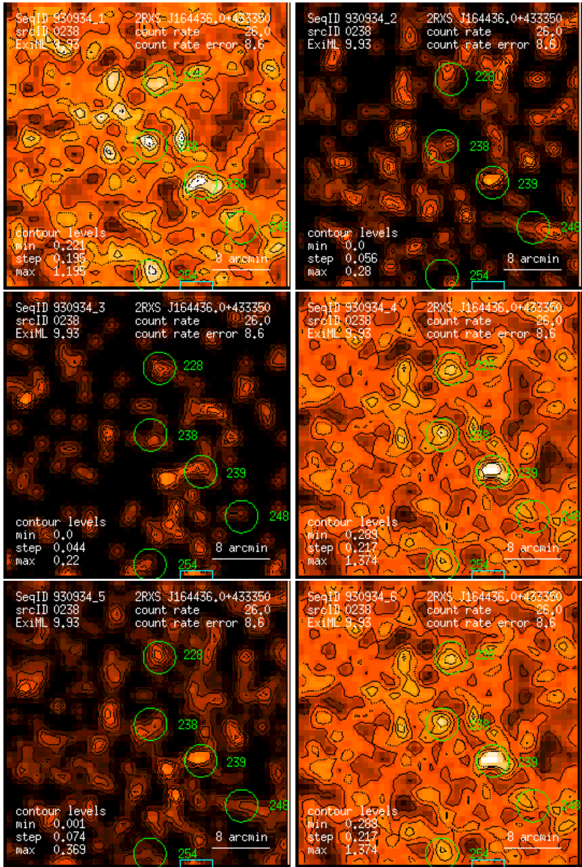
Figure 238: RASS 930934: detection 0238: band rate images, Gaussian filter: (1) PSPC channels 11 – 41, (2) 52 – 90, (3) 91 – 201, (4) 11 – 235, (5) 52 – 201, (6) 11 – 201. Broad band rates in counts/ks. Band rate contour levels in counts/ks/arcmin 2 .
