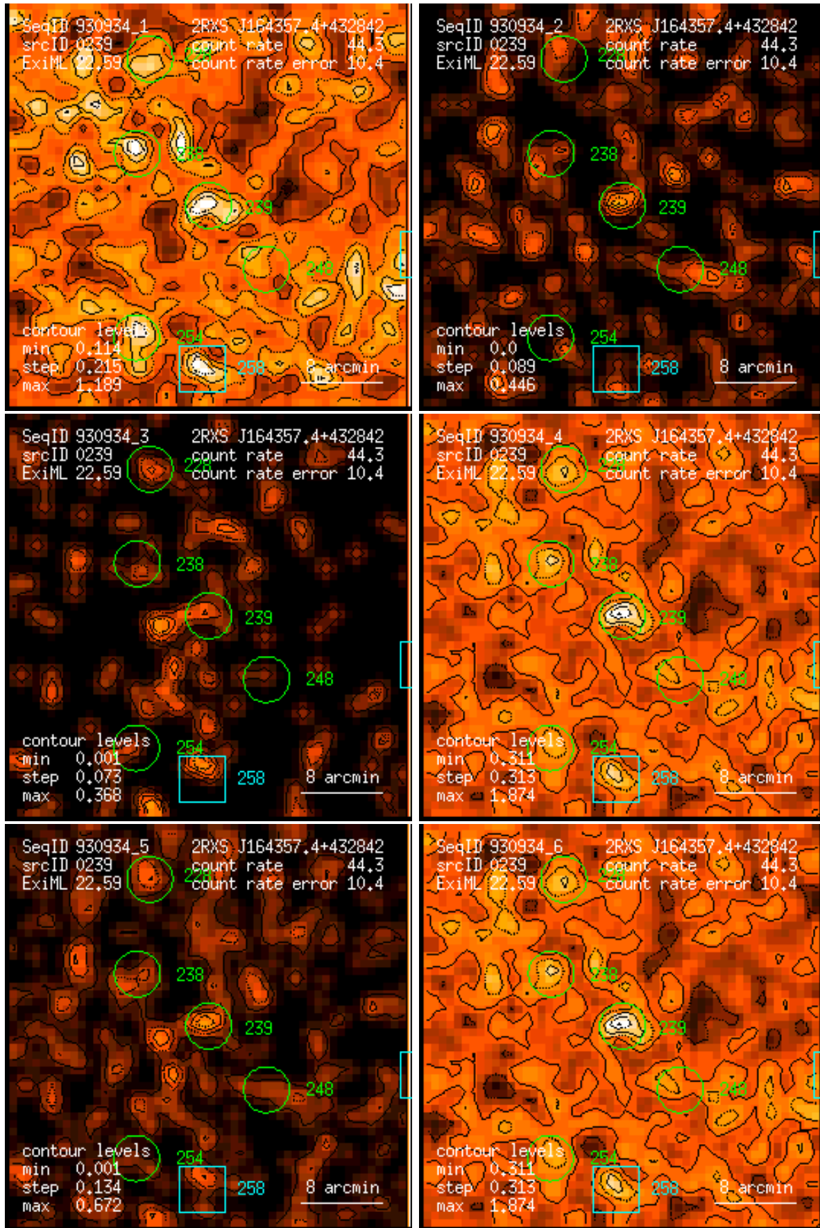
Figure 239: RASS 930934: detection 0239: band rate images, Gaussian filter: (1) PSPC channels 11 – 41, (2) 52 – 90, (3) 91 – 201, (4) 11 – 235, (5) 52 – 201, (6) 11 – 201. Broad band rates in counts/ks. Band rate contour levels in counts/ks/arcmin 2 .
