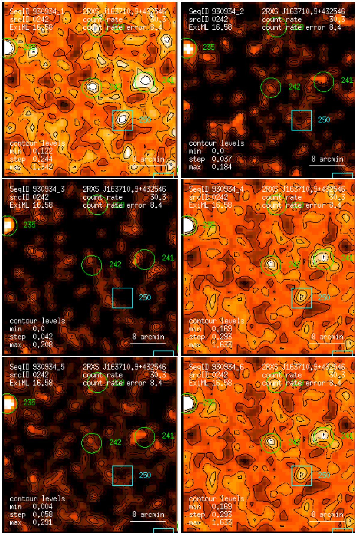
Figure 242: RASS 930934: detection 0242: band rate images, Gaussian filter: (1) PSPC channels 11 – 41, (2) 52 – 90, (3) 91 – 201, (4) 11 – 235, (5) 52 – 201, (6) 11 – 201. Broad band rates in counts/ks. Band rate contour levels in counts/ks/arcmin 2 .
