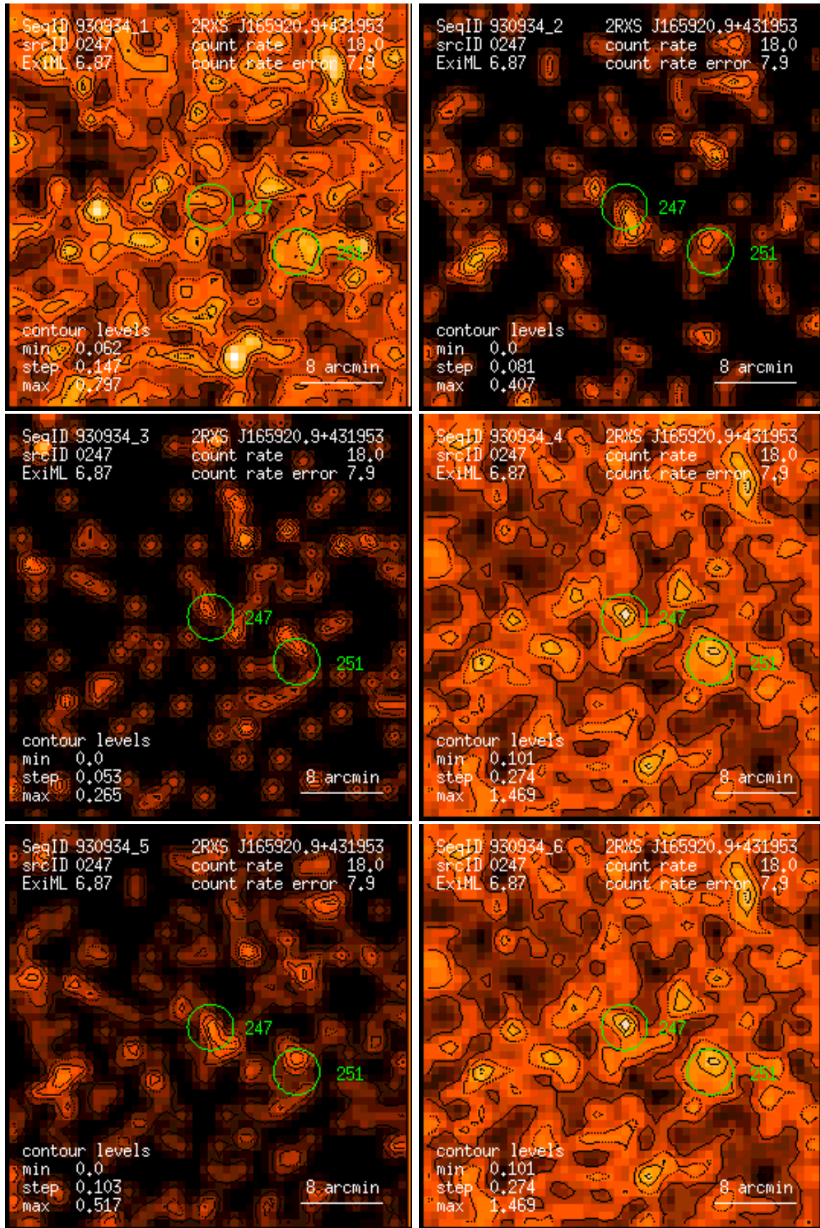
Figure 247: RASS 930934: detection 0247: band rate images, Gaussian filter: (1) PSPC channels 11 – 41, (2) 52 – 90, (3) 91 – 201, (4) 11 – 235, (5) 52 – 201, (6) 11 – 201. Broad band rates in counts/ks. Band rate contour levels in counts/ks/arcmin 2 .
